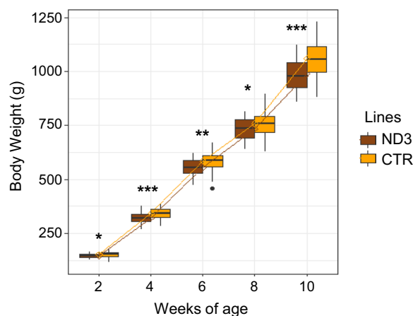
Fig. 5 Growth curve of ND3 and CTR chickens measured from 2 to 10 weeks of age. Asterisks indicate significant differences between lines at a given age (* p < 0.05 ; ** p < 0.01 ; *** p < 0.001 )
