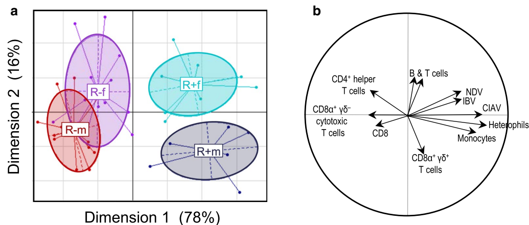
Fig. 4 a Projection of first and second axis of BGA based on white cell count and antibody titer data. Individuals are grouped and color-coded according to line (R+ and R-) and sex (m = males and f = females): R- m = red, R+ m = blue, R- f = purple, and R+ f = turquoise. b Representation of the partial contributions of cell types and antibodies to differentiation along the first two axes
