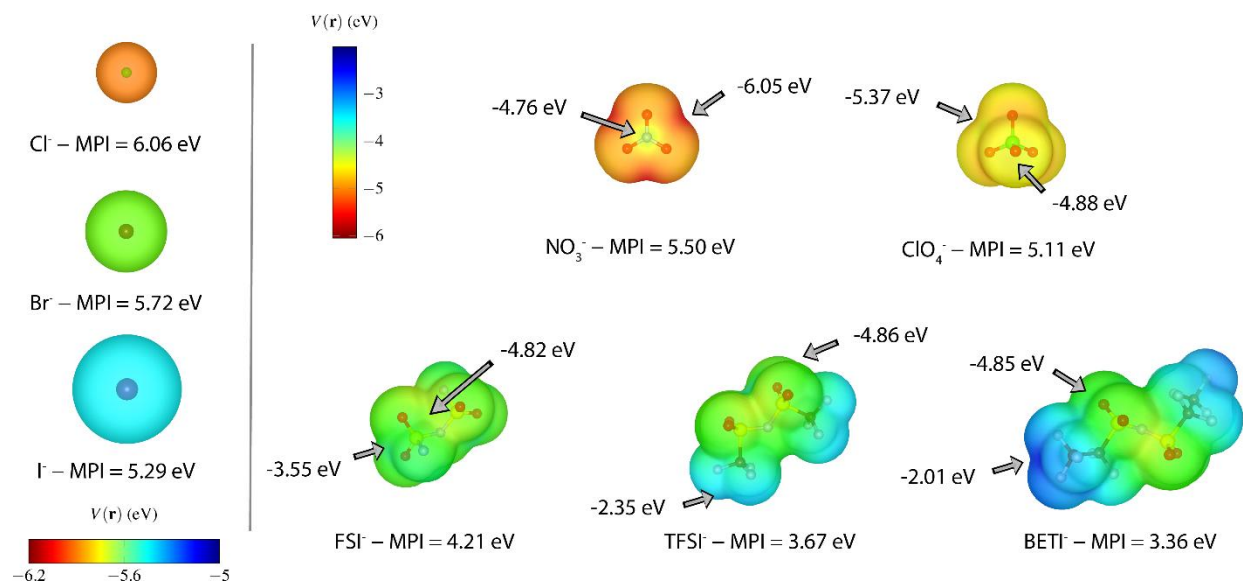
Figure 4. Electrostatic potential V(r) mapped to the 0.001 \text{ e}/\text{\AA}^3 isosurface of the electron density for a series of anions ( \text{Cl}^- , \text{Br}^- , \text{I}^- , \text{NO}_3^- , \text{ClO}_4^- , FSI, TFSI, BETI) obtained from gas phase quantum chemistry calculations (PBEo/ ma-def2-TZVP), along with the molecular polarity index (MPI). For non-spherical anions, extrema values of the electrostatic potentials are indicated along with their location on the isosurfaces.
