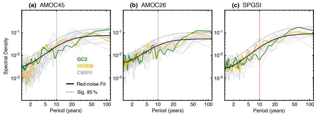
Figure 3. (a–c) Fourier spectra in the picontrl ensemble for the indices AMOC45, AMOC26, and SPGSI. Red noise spectra corresponding to a first-order autoregressive process fit to GC2 indices are provided as a reference.
