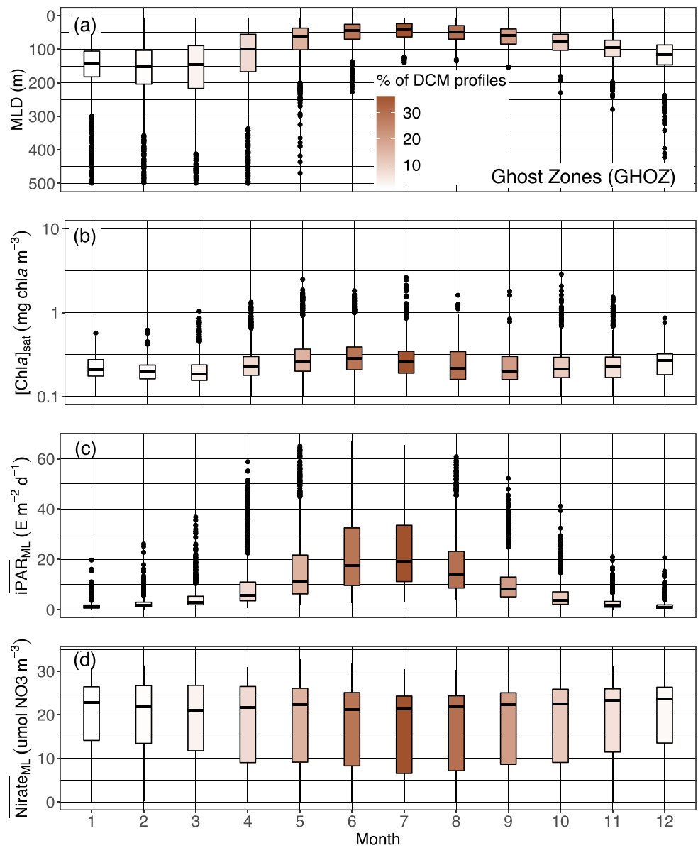
Figure 12. Quartile diagrams of (a) MLD, (b) [Chla]_{sat} , (c) mean daily PAR in the mixed layer ( \overline{iPAR_{ML}} ), and (d) mean nitrate concentration in the ML ( Nitrate_{ML} ) per Northern Hemisphere-phased month (regardless of the year) for GHZO profiles with a monthly occurrence of DCM profiles (color gradient). The North Atlantic Current is excluded from this representation, as not being part of the Southern Ocean sub-regions on which our analysis essentially focuses. DCM, Deep Chlorophyll Maximum; GHZO, Ghost Zone; MLD, Mixed Layer Depth; PAR, Photosynthetically Available Radiation.
