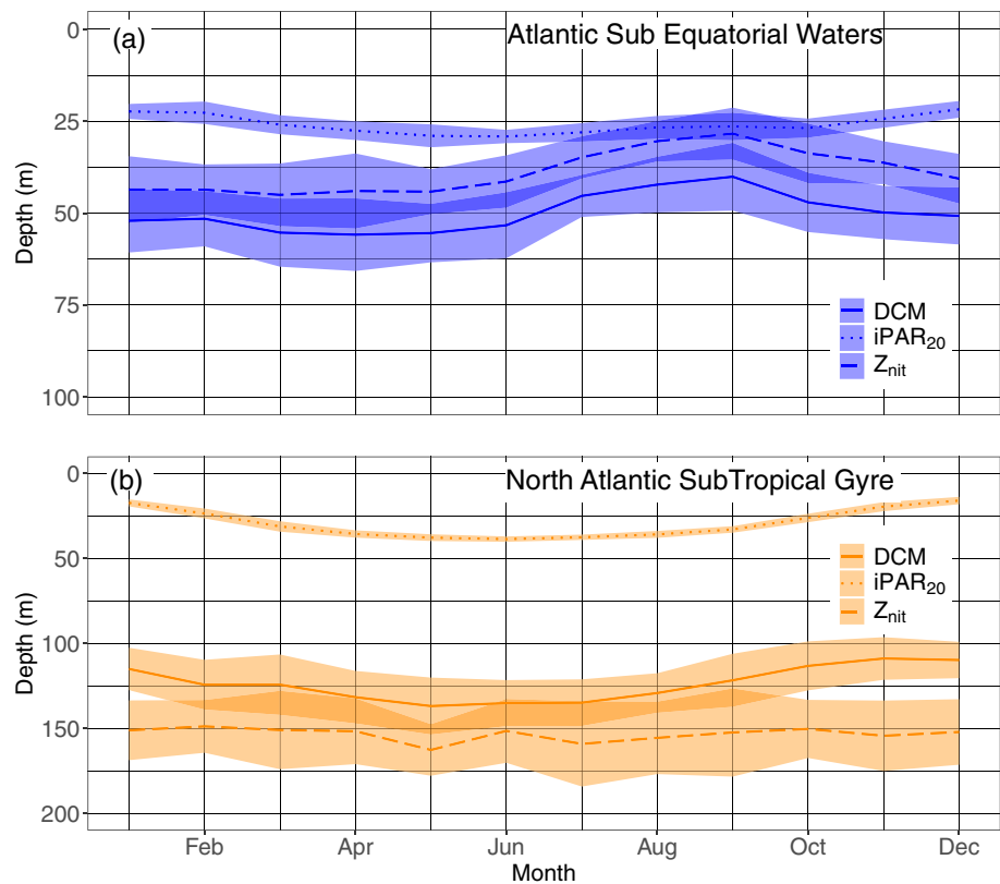
Figure 10. Mean and standard-deviation yearly climatology of the DCM depth, the depth of the iPAR\ 20\ E\ m^{-2}\ d^{-1} isocline and the nitracline depth for the floats in the Atlantic SubEquatorial Waters (a) and in the North Atlantic Subtropical Gyre (b), respectively, representative of the Deep Biomass Zone, and of the Deep photoAcclimation Zone. DCM, Deep Chlorophyll Maximum.
