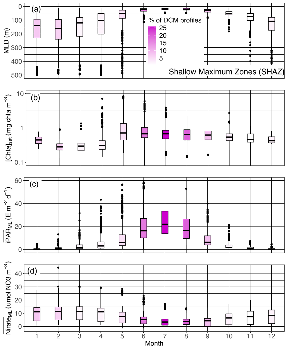
Figure 11. Quartile diagrams of (a) MLD, (b) [Chla]_{sat} , (c) mean daily PAR in the mixed layer ( \overline{iPAR_{ML}} ) and (d) mean nitrate concentration in the ML ( Nitrate_{ML} ) per Northern Hemisphere-phased month (regardless of the year) for SHAZ profiles with a monthly occurrence of DCM profiles color gradient. The Black Sea is excluded from this representation. DCM, Deep Chlorophyll Maximum; MLD, Mixed Layer Depth; PAR, Photosynthetically Available Radiation.
