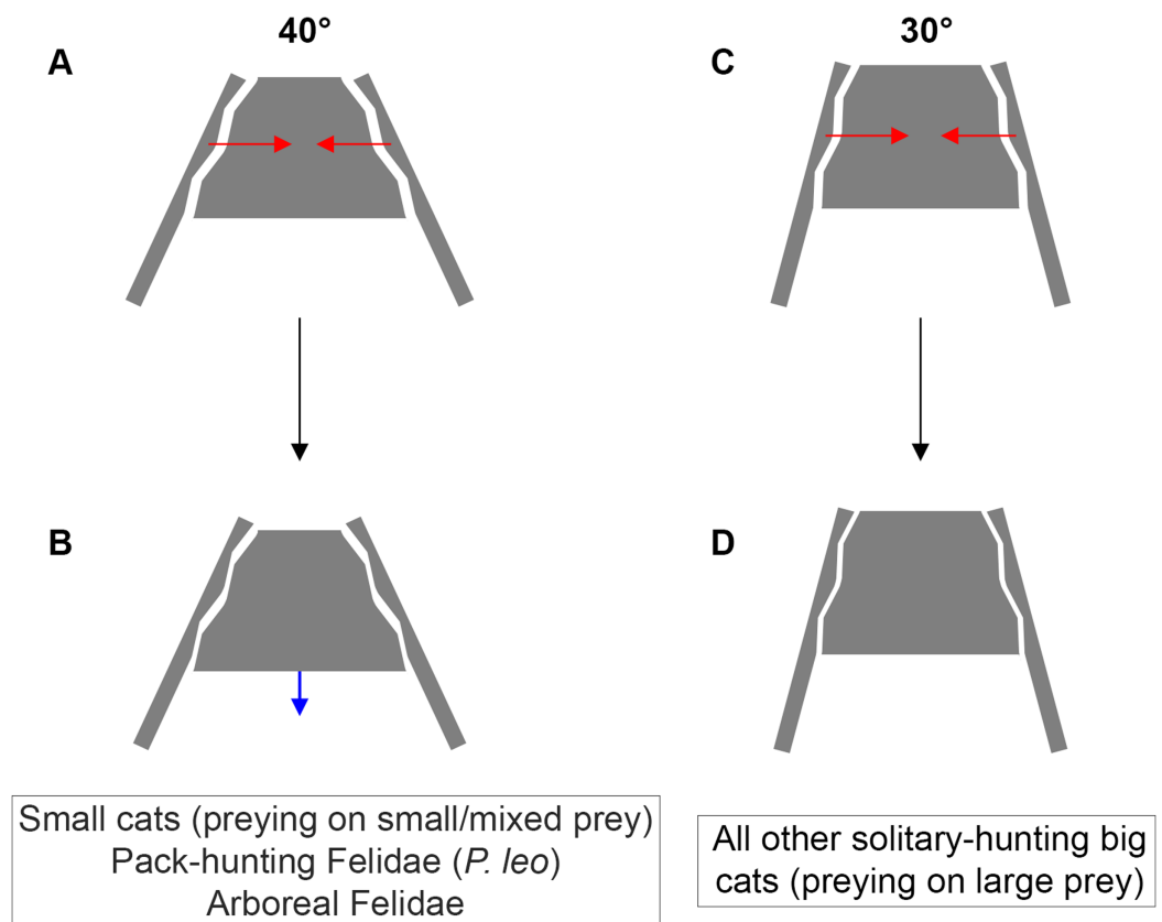
Figure 6 Inter-iliac angle in the interlocking process during predatory behavior in Felidae. (A–B) Predators with an angle of around 40° include solitary-hunting small cats, pack-hunting Felidae (lions) and arboreal Felidae. (C–D) Predators with an angle of around 30° include all solitary hunting big cats. The red arrows represent the forces produced through the post-cranial system and applied on the iliac wings (A, C). The blue arrow represents the possible slippage of the sacrum (B). We hypothesize that such movement is not possible for an inter-iliac angle of around 30° (D).
