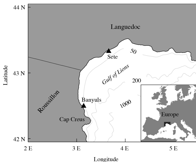
Fig. 1. – Map of the Gulf of Lions in Europe and bathymetric map of the Gulf of Lions with wave bouys locations in Banyuls (50 m, 3^{\circ}10.04 E, 42^{\circ}29.36 N) and Sète (30 m, 3^{\circ}39.55 E, 43^{\circ}19.70 N).
