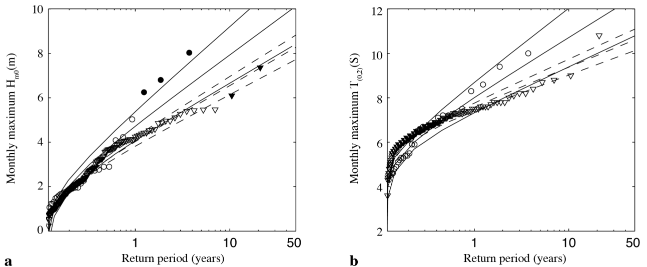
Fig. 4. – Cumulative probability distribution for wave height H_{m0} (a) and wave period T_{(0,2)} (b) in Banyuls: (o) raw data, (–) Gumbel fit and 80 % confidence interval, and in Sète: ( \nabla ) raw data, (–) Gumbel fit and 80 % confidence interval. The filled symbols display the largest wave heights recorded at both sites.
