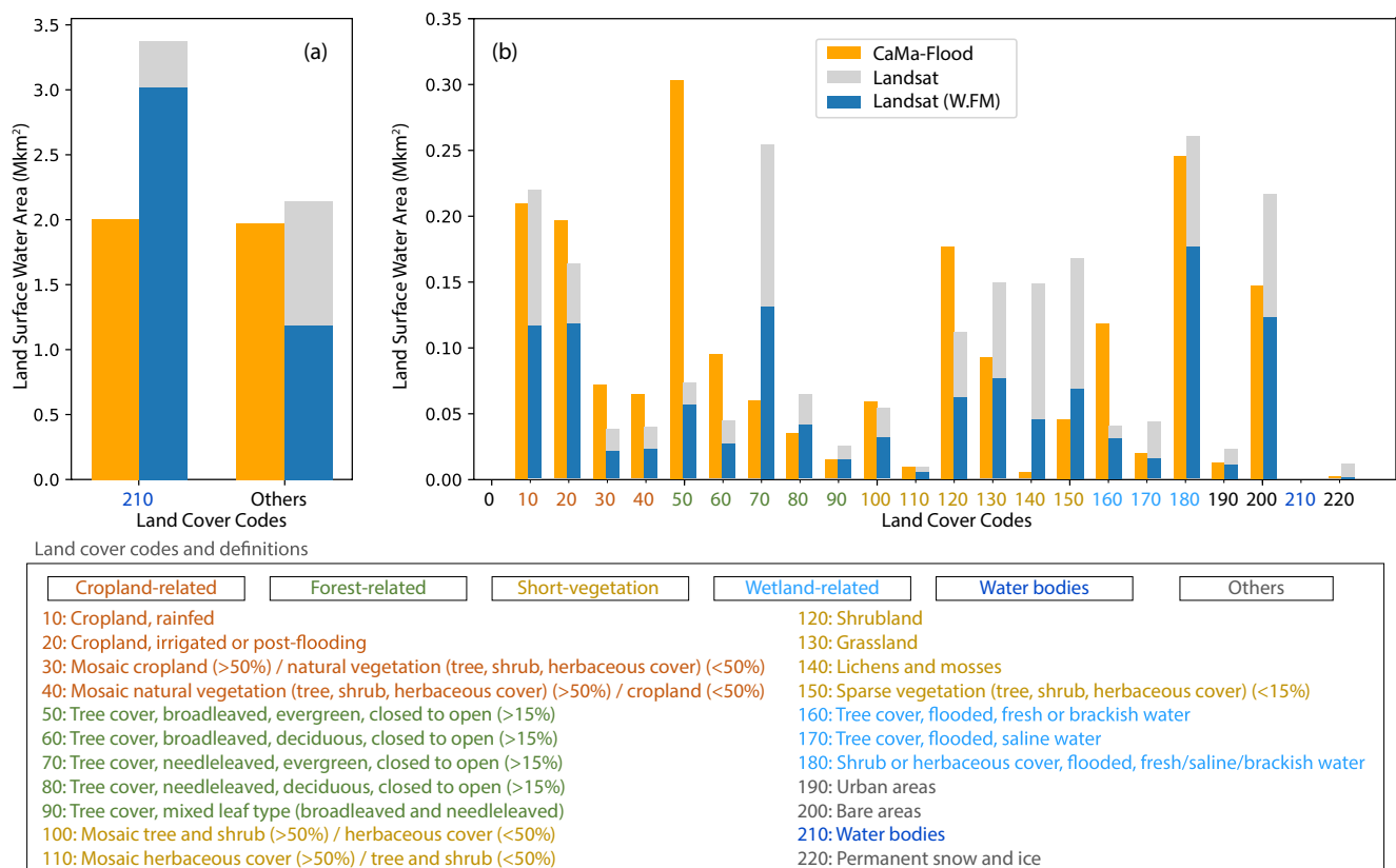
Figure 8. Comparison of LSWA among groups of land cover types. All land cover types other than water bodies ( cci\_code = 210 ) are grouped in the type “others” in (a). The orange bars represent the results of CaMa-Flood. The gray bars represent Landsat observations before application of the CaMa-Flood floodplain mask, and the blue section represents the results of Landsat after applying the floodplain mask. A list of cci\_code values and definitions of the land cover types is attached (ESA, 2017). All land cover types can be categorized as cropland-related land cover types, forest-related land cover types, short vegetation, wetland-related land cover types and others including water bodies (shown in different colors in the list and figure). CaMa-Flood, Catchment-based Macro-scale Floodplain model; LSWA, land surface water area.
