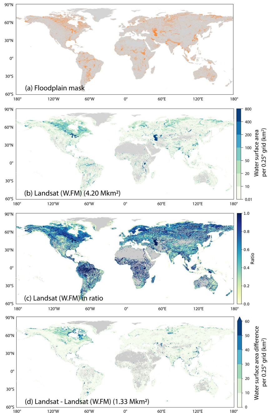
Figure 4. (a) Distribution of the CaMa-Flood floodplain mask over the globe (3"). (b) Landsat LSWA within the floodplain mask (named as Landsat (W.FM)). (c) The ratio of Landsat (W.FM) to total Landsat LSWA. (d) The difference in the value of Landsat (W.FM) from the total Landsat LSWA. b, c and d are illustrated at 0.25° resolution for better visualization. The values are for each 0.25° by 0.25° grid. CaMa-Flood, Catchment-based Macro-scale Floodplain model; LSWA, land surface water area.
