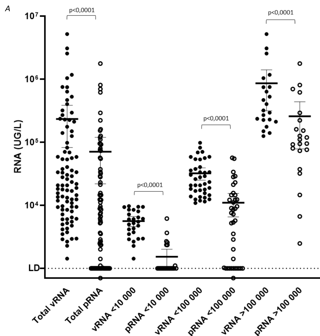
Figure 4. Relative proportion of protected vs unprotected SARS-CoV-2 genomes in raw wastewaters collected in Greater Paris area. Raw wastewater samples (n=87) from four WWTP were analyzed for SARS-CoV-2 genome by RT-qPCR (vRNA, filled circle) and using integrity assay (pRNA, open circle). The concentration (UG/L) was plotted on the panel A, the median values and interquartiles (25-75%) are indicated. The pRNA/vRNA ratio indicating the percentage of protected RNA over total viral RNA, is plotted for each sample on panel B. The median values and interquartiles (25-75%) are indicated.
