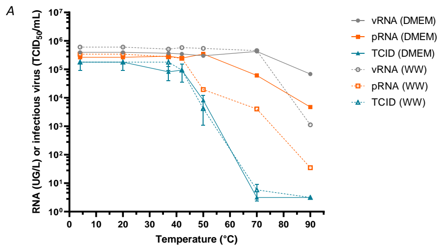
Figure 3. Stability to heat of total viral RNA, protected viral RNA and infectious SARS-CoV-2 and coxsackievirus B5 in spiked wastewater. Wastewater samples were spiked with infectious CV-B5 particles (panel A) or infectious SARS-CoV-2 particles (panel B) and incubated for 10 min at various temperatures. Total viral RNA (vRNA) was quantified by RT-qPCR, protected RNA (pRNA) was quantified by an integrity-based RT-PCR, as described, and infectious virus (TCID 50 ) was titrated by cell culture.
