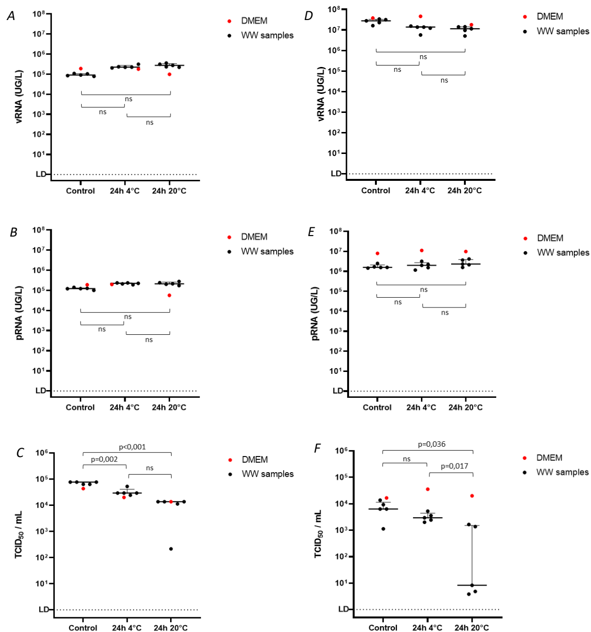
Figure 2. Stability of total viral RNA, protected viral RNA and infectious SARS-CoV-2 and coxsackievirus B5 in spiked wastewater samples. Five wastewater samples were spiked with infectious virus and incubated for 24h at +4°C or +20°C. DMEM was used as a control of matrix. Total viral RNA (vRNA) of CV-B5 (panel A) or SARS-CoV-2 (panel D) were quantified by RT-qPCR. Protected RNA (pRNA) of CV-B5 (panel B) or SARS-CoV-2 (panel E) were quantified using an integrity-based RT-PCR, as described. Infectious particles (TCID 50 ) of CV-B5 (panel C) or SARS-CoV-2 (panel F) were titrated by cell culture.
