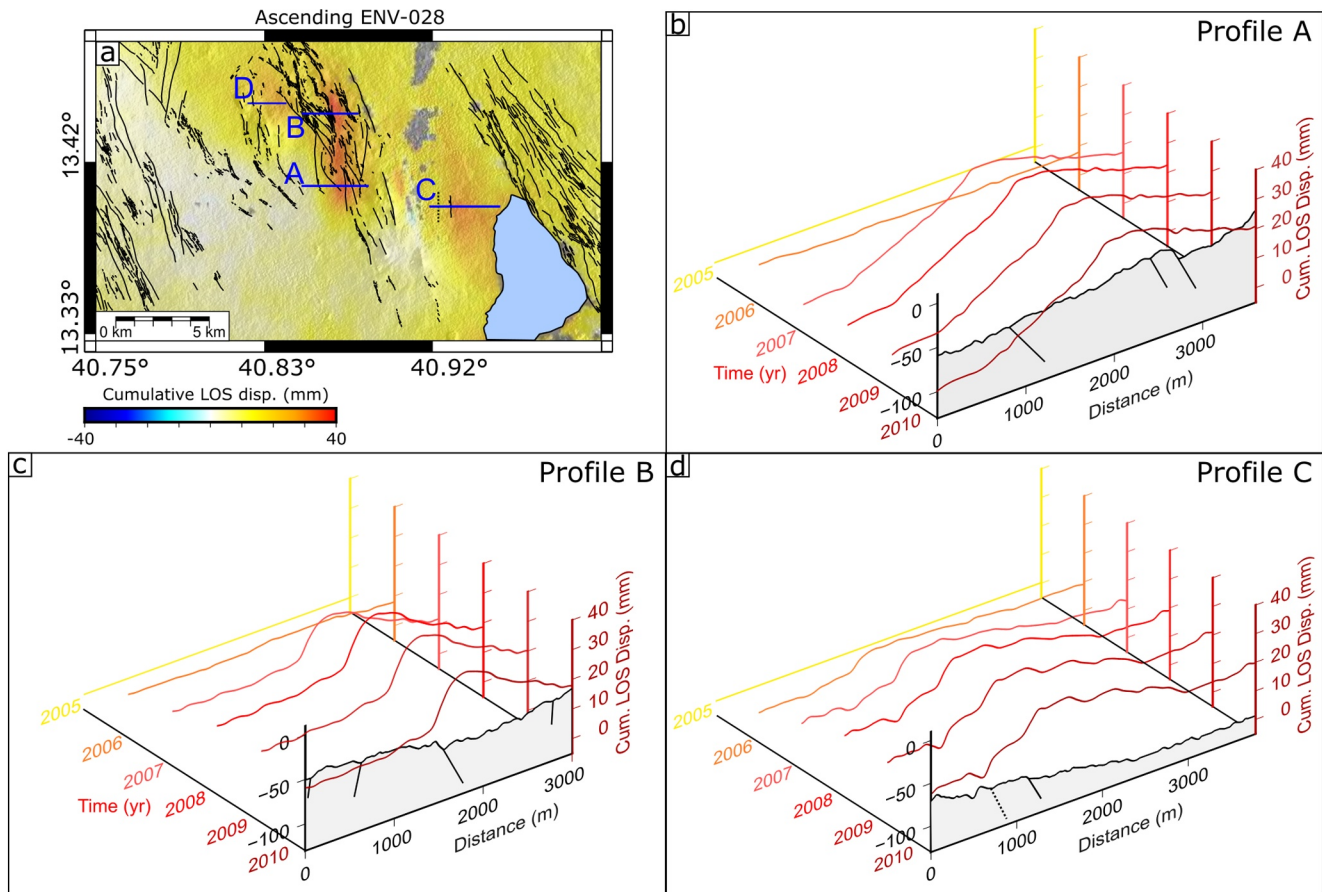
Figure 4. ENVISAT time-series of cumulative LOS displacements and active faults along different profiles. (a) Locations of profiles in ascending track 028 and mapped faults (black lines). The time-series clearly shows that both sudden ((b) and (c)) and time-progressive deformation (d) occur corresponding to the faults. The major faults that were mapped are also shown in cross section (black lines). Further time-series are shown in Figure S6.
