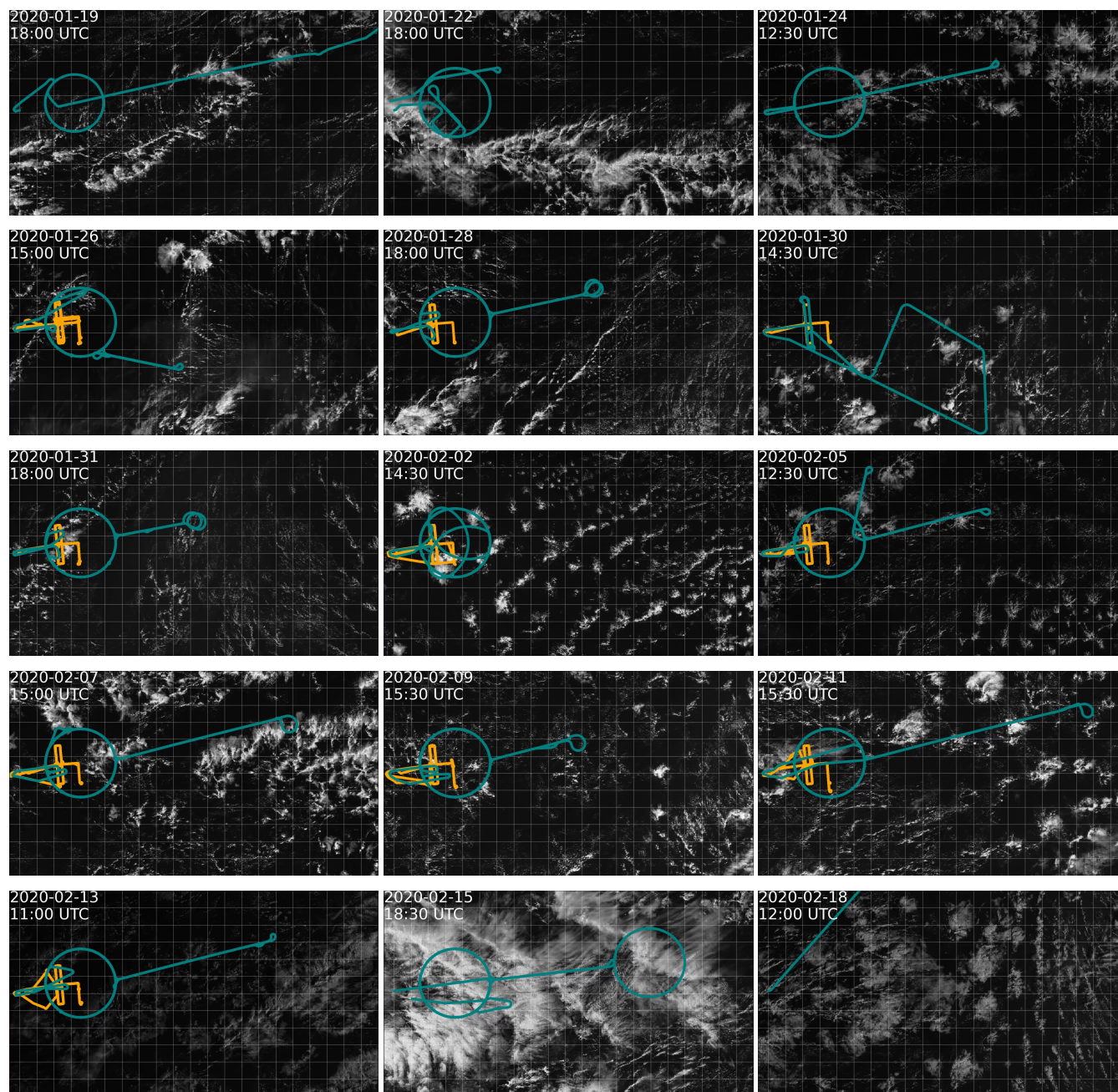
Figure 3. Snapshots of animations of GOES-16 ABI images (channel 2; 0.64 \mu\text{m} ) for all flights. Tracks of the HALO and ATR aircraft are indicated in teal and orange, respectively. Snapshots are from about mid-flight time of HALO, except for the ferry flights.
