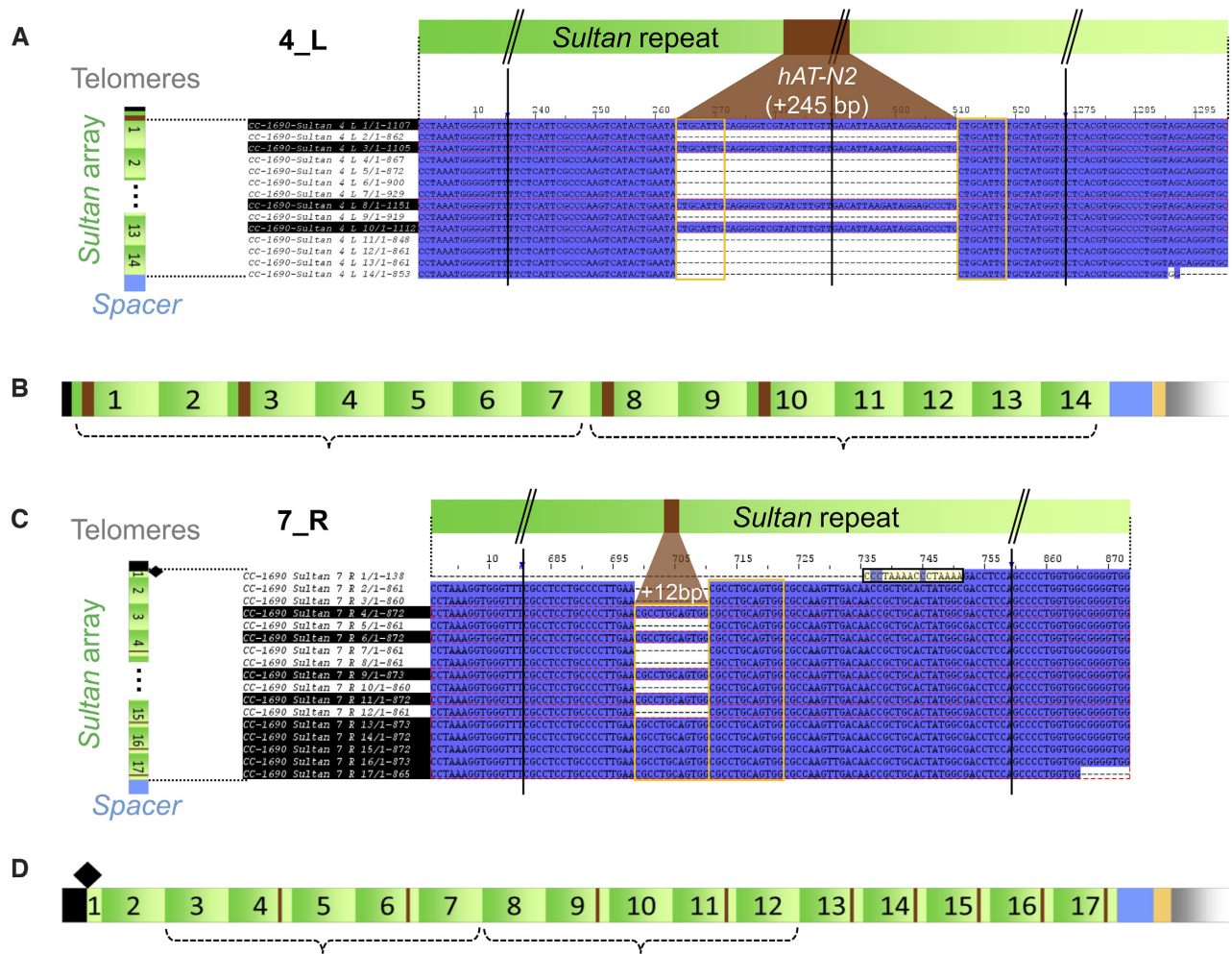
Figure 3. Evidence for multiple-copy duplication events in Sultan arrays. (A) and (C) Alignment of Sultan repeat sequences from class A subtelomeres 4.L and 7.R, from the telomere-proximal (top) to the Spacer -proximal (bottom). Conservation of nucleotide across repeats is indicated in dark blue. Vertical black bars and ‘/’ denote sequence portions not shown. Sultan repeats highlighted in black present a large insertion, represented in brown. Orange frames highlight duplications (including a putative hAT-N2 8-bp target-site duplication in 4.L). In (C), the end of the telomere is highlighted in yellow. (B) and (D) Sketch of 4.L and 7.R Sultan arrays with the conserved insertions (brown). Dotted brackets indicate multi- Sultan segments likely duplicated ‘en bloc’ on each subtelomere.
