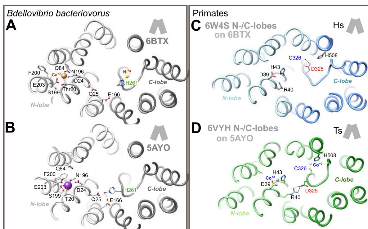
Figure 4. Predicted arrangement of the N- and C-lobes of the HsFPN1/TsFpn in an inward-facing conformation (panels C and D), as deduced from superimposition of the N- and C-lobes of the HsFPN1/TsFpn in an outward-facing conformation onto the corresponding lobes in the 3D structures of BbFpn solved in an inward-facing conformation (panels A and B). H-bonds and salt-bridges are shown with dashed lines. The BbFpn/TsFpn 3D structures also illustrate the position and features of the ion binding sites in the N-lobes.
