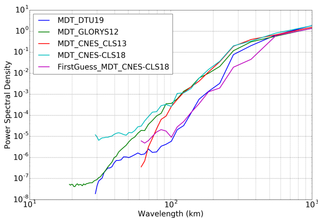
Figure 7. Meridional spectral power density obtained for different MDT solutions in a 10^\circ box centered around ( 49^\circ S, 43^\circ E).
