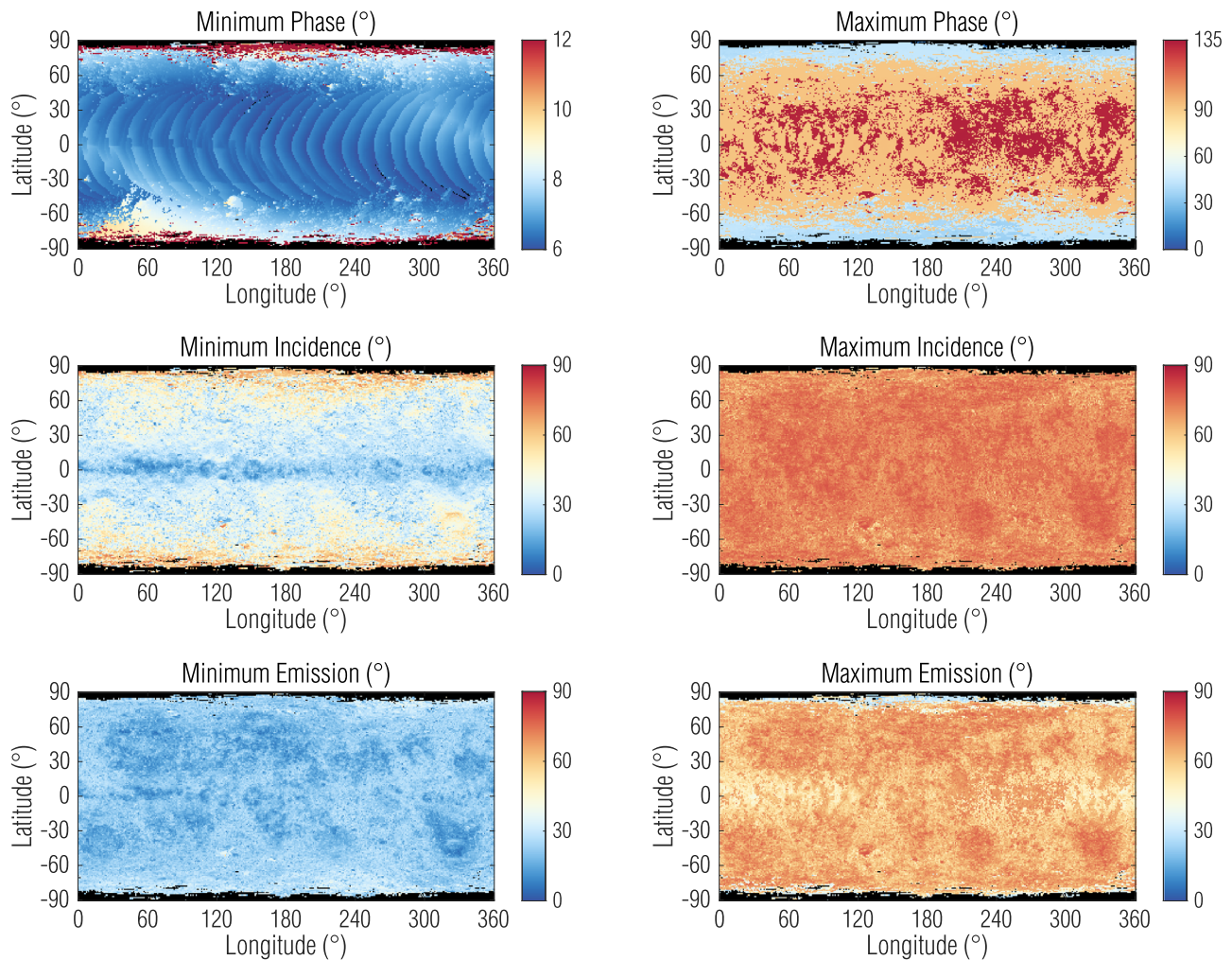
Figure 1. Maps of emission, incidence, and phase angle indicate extensive photometric angle coverage across Benu’s surface in the v filter. The other MapCam filters have nearly identical coverage.
