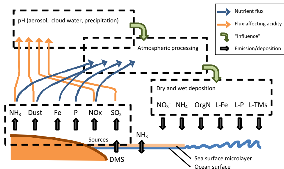
Fig. 1. Overview of the atmospheric acidity, nutrient, and trace element cycles. Emissions of \text{NH}_3 , \text{NO}_x , \text{SO}_2 , and dust influence atmospheric acidity (orange arrows). Dust, anthropogenic trace element emissions (abbreviated as Fe), and anthropogenic and biological sources of P, \text{NH}_3 , and \text{NO}_x contribute to the atmospheric nutrient/trace element burden (blue arrows). The majority of sources are terrestrial, although ship-based emissions of Fe and \text{NO}_x are important and marine emissions of dimethyl sulfide (DMS) are a substantial source of \text{SO}_2 , particularly in the Southern Hemisphere. Acidity-driven atmospheric processing alters the labile nutrient flux to the ocean, either by affecting the gas-aerosol partitioning or by altering the labile fractions of Fe (L-Fe), P (L-P), and trace metals (L-TM). Organic nitrogen compounds (OrgN) are also generated during atmospheric processing but are not discussed here.
