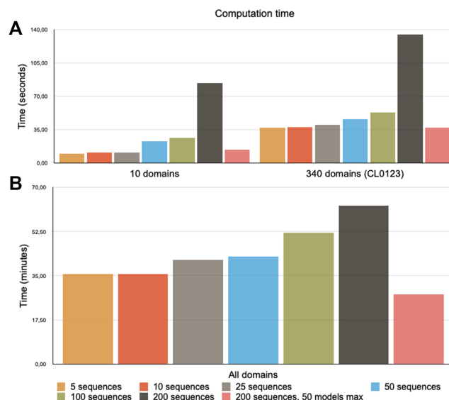
Figure 2. Performance analysis. MyCLADE time performance is evaluated on sets of sequences of various size with (A) either 10 domains, or 340 domains belonging to the largest Pfam clan CL0123 (in seconds) or (B) with all Pfam domains (in minutes). A dataset of 200 sequences, of length varying from 494 aa up to 671 aa, has been constructed from the Harmonizome database and three different subsets of 5, 10, 25, 50 and 100 sequences have been randomly extracted from it and tested. The plot reports the computing time needed for MyCLADE annotation without DAMA averaged over the three datasets for each experiment. The sets have been evaluated with the complete library of models (<350 models per domain) and with a reduced library (<50 models per domain).
