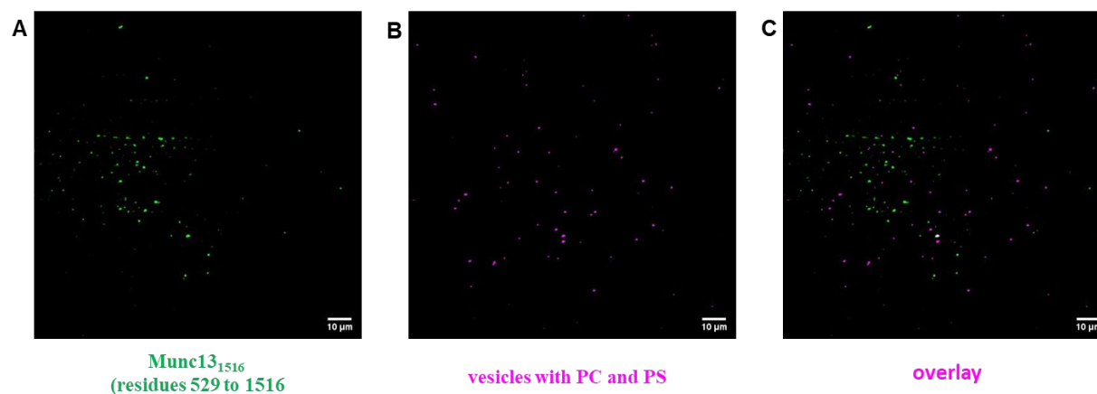
Fig. S6. Deletion of the hydrophobic end of MUN domain further reduces Munc13-1's function of capturing vesicles. (A) TIRF image of clusters formed by Munc13 1516 (residues 529 to 1516) labeled with Alexa488 on lipid bilayer. (B) TIRF image of vesicles containing PC and PS that are anchored to lipid bilayer. (C) Merge of the previous two images, which shows that Munc13 1516 clusters capture fewer vesicles in the absence of C 2 C domain.
