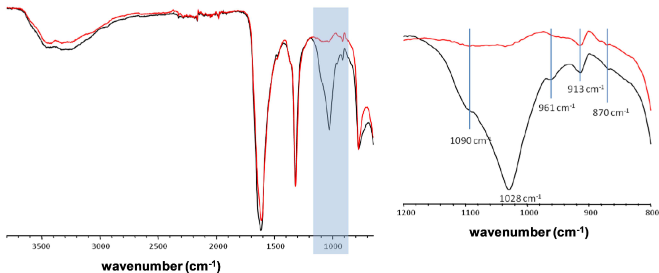
Figure A1. FTIR spectra of two KS containing a mixture of COM and COD phases. The main difference lies in the light blue 460 wavenumber region corresponding to phosphate vibrations (including hydroxyapatite: 913, 961, 1090 \text{cm}^{-1} , carbonates: 870 \text{cm}^{-1} ).
