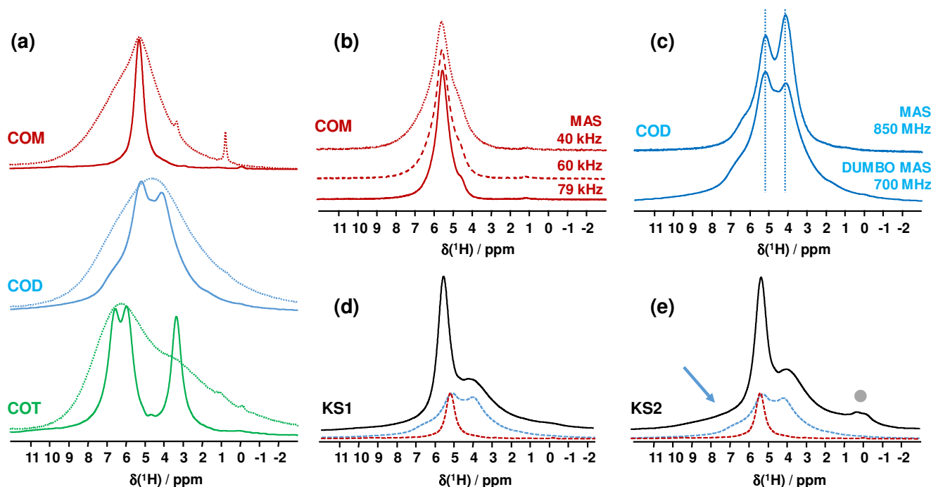
110 Figure 1. (a) ^1\text{H} MAS (dashed lines) and ^1\text{H} DUMBO MAS (solid lines) NMR spectra of COM (in red), COD (in blue), COT (in green) ( \nu_{\text{rot}} = 12 kHz, 700 MHz, 16.4 T). Only the isotropic resonances are represented. (b) ^1\text{H} very-fast MAS (40, 60 and 79 kHz) NMR spectra of COM at very high magnetic field (850 MHz). (c) Comparison of the ^1\text{H} NMR spectra of COD obtained under DUMBO MAS ( \nu_{\text{rot}} = 12 kHz, 700 MHz) and very-fast MAS ( \nu_{\text{rot}} = 79 kHz, 850 MHz) conditions. Vertical dashed lines are guidelines for the eyes. (d) ^1\text{H} DUMBO MAS NMR spectrum of KS1 ( \nu_{\text{rot}} = 12 kHz, 700 MHz). The red and blue dashed lines correspond to experimental ^1\text{H} DUMBO MAS NMR spectra of COM and COD, respectively. (e) ^1\text{H} DUMBO 115 MAS NMR spectrum of KS2 ( \nu_{\text{rot}} = 12 kHz, 700 MHz). The plain light grey circle indicates the presence of organic
