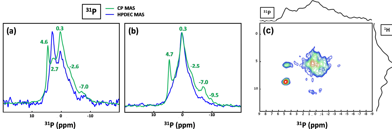
Figure 9. (a) ^{31}\text{P} MAS under high power \{^1\text{H}\} decoupling (in blue) and CP MAS (in green) NMR spectra of KS4. Some 365 specific chemical shifts are highlighted. (b) ^{31}\text{P} MAS under high power \{^1\text{H}\} decoupling (in blue) and CP MAS (in green) NMR spectra of KS5 (representative of an ensemble of five KS). Some specific chemical shifts are highlighted. (c) ^1\text{H} - ^{31}\text{P} HETCOR CP MAS NMR spectrum of KS4 (temperature control at -20^\circ\text{C} ). All spectra shown here were recorded at 16.4 T.
