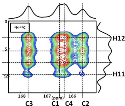
Figure A2. ^1\text{H} - ^{13}\text{C} CP DNP MAS NMR spectrum of COM at T = 100 K. Four distinct ^1\text{H} resonances are clearly evidenced on the ^1\text{H} indirect dimension. The contact time is 9.0 ms and sixteen ^1\text{H}/^{13}\text{C} correlations are observed.
