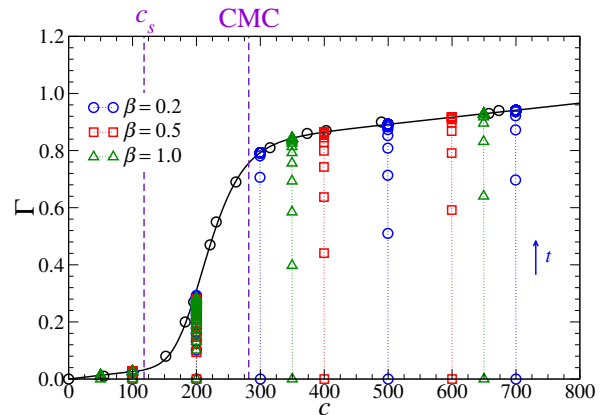
FIG. 4. Cooperative adsorption model for the adsorption of TX100 surfactants onto silica (all details can be found in Ref. [32]). The adsorbed amount is expressed as the surface concentration \Gamma as a function of the bulk concentration c . The black solid line denotes the theoretical adsorption isotherm as predicted using the cooperative model while the black circles denote the experimental data. The colored symbols correspond to the kinetic results obtained using the Lattice Boltzmann calculations. The different colors denote the results of the cooperative model with different aggregation constants: \beta = 0.2 (blue), \beta = 0.5 (red), and \beta = 1.0 (green). Each dotted line indicates the time evolution of the adsorbed amount \Gamma(t) for a specific aggregation constant \beta and an initial concentration c_0 . c_s is the surface aggregation concentration while CMC is the critical micelle concentration.
