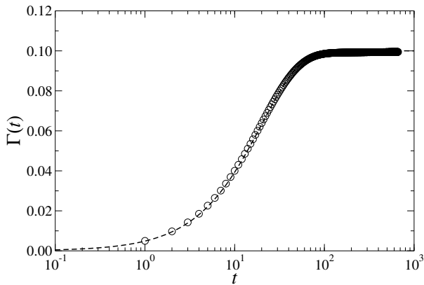
FIG. 3. Comparison between the adsorption kinetics \Gamma(t) predicted using Lattice Boltzmann simulations and the analytical expression for the Henry adsorption regime. These data are obtained for an adsorption isotherm corresponding to the Henry regime with a Henry constant k_H = 0.01 ( p_A = 0.0005 and p_D = 0.05 ). The initial concentration is c_0 = 10 . The open symbols correspond to the numerical solution using the Lattice Boltzmann model while the dashed line indicates the analytical expression for Henry kinetics as described in Eq. (9).
