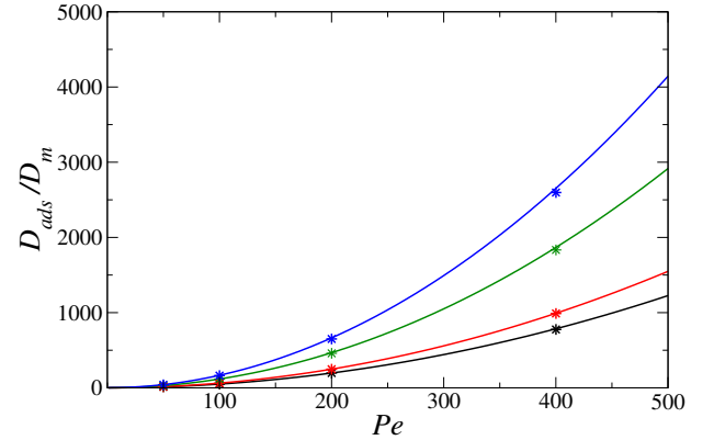
FIG. 6. Normalized dispersion coefficient for adsorbing molecules carried in a slit pore geometry by a liquid flow (obeying a simple Poiseuille flow). The data are presented as a function of the Peclet number which characterizes the diffusion/advection rate. Adsorption is described using a simple Henry law with different Henry constants k_H . The symbols correspond to the results from the Lattice Boltzmann calculations using the adsorption scheme. The data show D_{ads}/D_m = D(t \rightarrow \infty)/D_m where D(t) corresponds to the derivative of the displacement variance with respect to time. The lines correspond to the analytical expression for D_{ads}/D_m as derived by Levesque et al. [see Eq (24) in main text]. Different k_H are considered but, in all cases, a fixed desorption rate p_D = 0.01 is used. The red, black, green and blue symbols denote data obtained for k_H = 0.1, 1, 5 and 10 , respectively.
