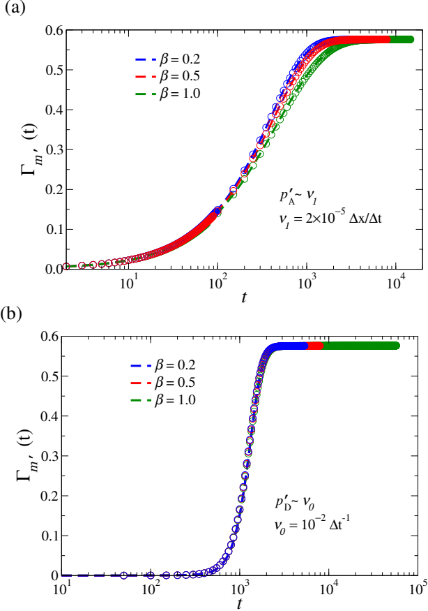
FIG. 5. Comparison between the adsorption kinetics predicted using the Lattice Boltzmann simulations and the analytical expression for the cooperative adsorption model for TX100 on silica for an initial concentration c_0 = 250 . The dashed lines denote the adsorption kinetics as determined by solving numerically Eq. (18). In more detail, these data show \Gamma_{m'} as a function of time t . The open symbols correspond to the numerical results obtained using the lattice Boltzmann model. For each data set, the colors denote the results from the cooperative model with different aggregation constants: \beta = 0.2 (blue), \beta = 0.5 (red), and \beta = 1.0 (green). Panel (a) corresponds to data with p'_A \sim \nu_1 and p'_D \sim \nu_1/k' while panel (b) corresponds to data with p'_A \sim \nu_0 k' and p'_D \sim \nu_0 .
