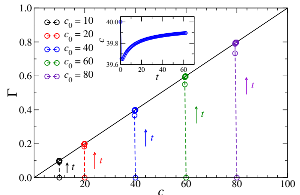
FIG. 2. Henry adsorption isotherm \Gamma(c) for a Henry constant k_H = p_A/p_D = 0.01 with p_A = 0.0005 and p_D = 0.05 . The adsorbed amount corresponds to the surface concentration \Gamma . The black solid line is the theoretical prediction \Gamma = k_H c while the open circles are the results from the Lattice Boltzmann calculations. Each color corresponds to a given initial concentration c_0 as indicated in the graph. For each color, the dashed line presents the time evolution of the adsorbed amount \Gamma(t) . The insert shows the concentration of free tracers in the adsorbing sites as a function of time.
