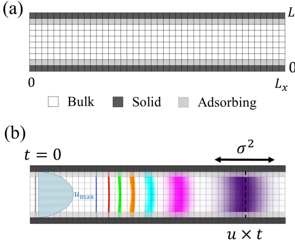
FIG. 1. Schematic representation of the simulation setup used in our Lattice Boltzmann calculations. (a) A slit pore having a length L_x and a width L is used as a simple reference system to validate our Lattice Boltzmann method. In the geometry mesh shown here, each site is either a fluid site (white) or a solid site (black). Fluid sites directly in contact with a solid site adsorb tracers (grey). (b) The molecule concentration within the geometry is monitored as a function of time t . These molecules are carried along the pore direction by a flowing liquid whose velocity field corresponds to Stokes flow (corresponding for this simple pore geometry to a Poiseuille velocity profile with a maximum velocity u_{max} ). Starting from a concentration peak injected at a given time t = 0 in a slice located in x_0 , the density broadens as molecular diffusion leads to tracer dispersion within the pore. The different colors denote different times which increase from left to right as the carrying fluid is transported along this direction). Under laminar flow conditions, the concentration distribution in the long time limit is given by Taylor regime where tracer dispersion leads to a concentration distribution with a Gaussian shape.
