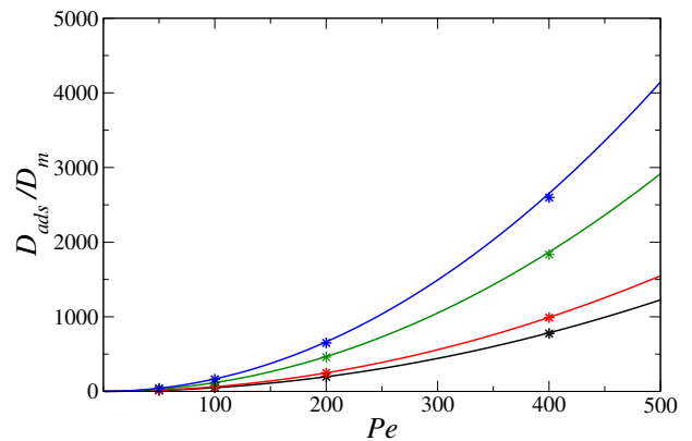
FIG. 6. Normalized dispersion coefficient for adsorbing molecules carried in a slit pore geometry by a liquid flow (obeying a simple Poiseuille flow). The data are presented as a function of the Peclet number which characterizes the diffusion/advection rate. Adsorption is described using a simple Henry law with different Henry constants k_H . The symbols correspond to the results from the Lattice Boltzmann calculations using the adsorption scheme. The data show D_{ads}/D_m = D(t \rightarrow \infty)/D_m where D(t) corresponds to the derivative of the displacement variance with respect to time. The lines correspond to the analytical expression for D_{ads}/D_m as derived by Levesque et al. [see Eq (24) in main text]. Different k_H are considered but, in all cases, a fixed desorption rate p_D = 0.01 is used. The red, black, green and blue symbols denote data obtained for k_H = 0.1, 1, 5 and 10 , respectively.
