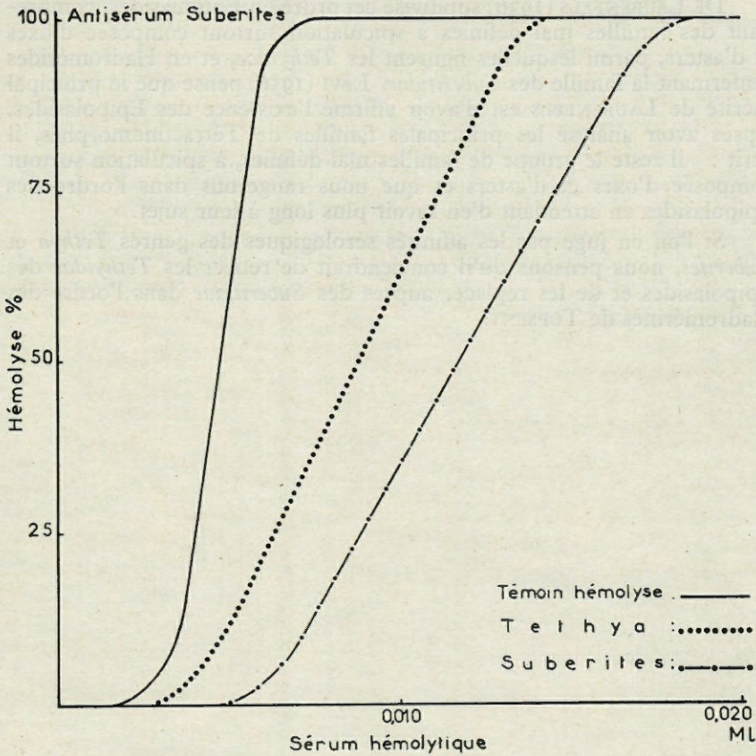
Courbe II.
