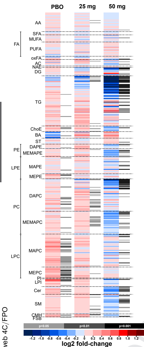
Figure 4. Lipidomic profiling of patient serum. (A) Lipidomic profiling of 400 species performed by UHPLC-MS. Heatmap of binary paired comparisons of week 12 to baseline for placebo ( n = 25 ), 25 mg TVB-2640 ( n = 27 ), and 50 mg TVB-2640 ( n = 28 ) as \log_2 pairwise fold change. Lipids are grouped by class as indicated for a total of approximately 400 species. Red indicates increase and blue indicates decrease. Statistical significance is indicated in gray scale for each species. (B) Heatmap displaying the changes (week 12 compared to baseline) in TG species with respect to number of carbons and double bonds. Color code represents the transformed ratios between means of the groups ( \log_2 [fold-change]). Student t test P values (or Welch's t test where unequal variances were found): * P < .05 ; ** P < .01 ; *** P < .001 . AA, amino acids; AC, acyl carnitines; ArAA, aromatic amino acids; BA, bile acid; BCAA, branched chain amino acids; Cer, ceramides; ChoE, cholesteryl ester; CMH, monohexosylceramides (Cerebrosides); DAPE, diacylglycerophosphatidylethanolamines (DAPE); DAPC, diacylglycerophosphatidylcholines; DG, diglycerides; FSB, free sphingoid base; LPC, lysophosphatidylcholines; LPE, lysophosphatidylethanolamines; LPI, lysophosphatidylinositols; MAPC, monoacylglycerophosphocholines; MAPE, monoacylglycerophosphoethanolamine; MAPI, monoacylglycerophosphoinositol; MEMAPC, 1-ether, 2-acylglycerophosphocholines; MEMAPE, 1-ether, 2-acylglycerophosphoethanolamine; MEPC, monoetherglycerophosphocholines; MEPE, 1-monoetherglycerophosphoethanolamine; MUFA, monounsaturated fatty acid; NAE, N-acyl ethanolamines; NEFA, nonesterified fatty acid; PC, phosphatidylcholines; PE, phosphatidylethanolamine; PG, phosphatidylglycerols; PI, phosphatidylinositols; PUFA, polyunsaturated fatty acids; SFA, saturated fatty acid; SM, sphingomyelin; TG, triglycerides; UFA, unsaturated fatty acid.
