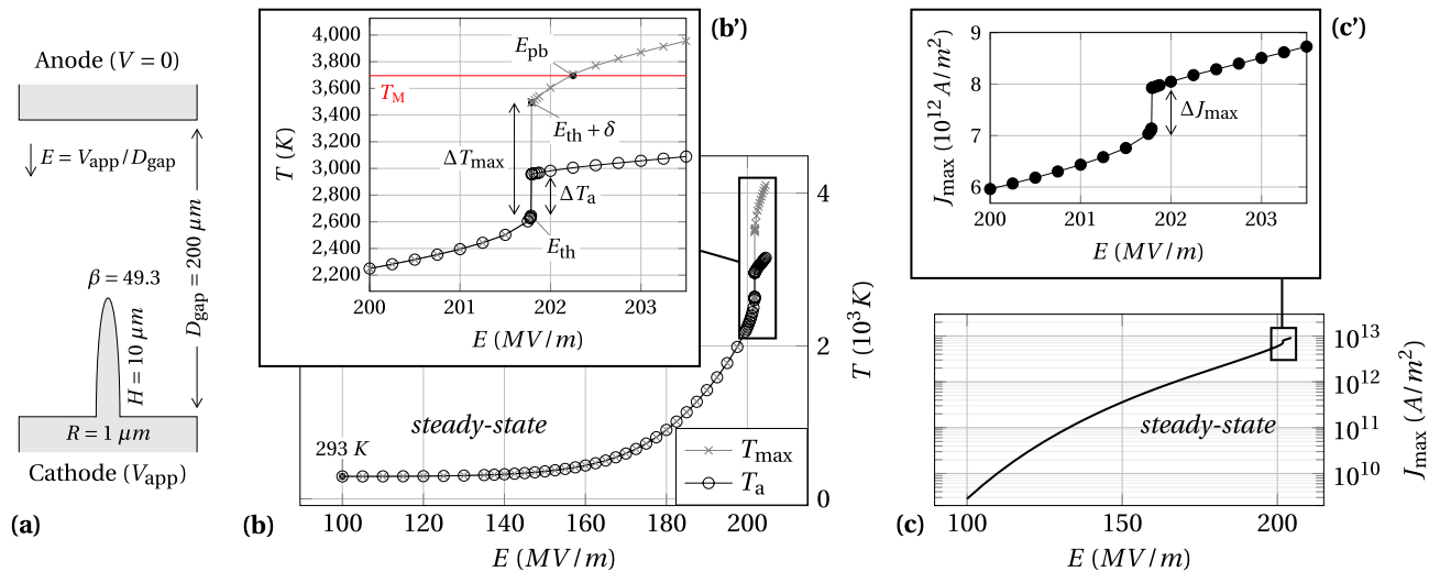
Figure 2. Highlight of a temperature jump versus the applied electric field in the steady state thermo-field emission of a tungsten hemieipsoid. (a) Sketch of the emitter. \beta is the apex field enhancement factor, so that the locally enhanced electric field at the apex is F = \beta E , where E is the applied electric field. The dimensions are not at scale. (b) Variation of the emitter maximum temperature T_{\max} and its apex temperature T_a versus the applied electric field. (c) Variation of the maximum emitted current density J_{\max} versus the applied electric field. Each data point is the result at steady state of a transient simulation where the field is raised from zero to the indicated x-axis value over a few nanoseconds. (b',c') are zooms of (b,c) framed areas, respectively.
