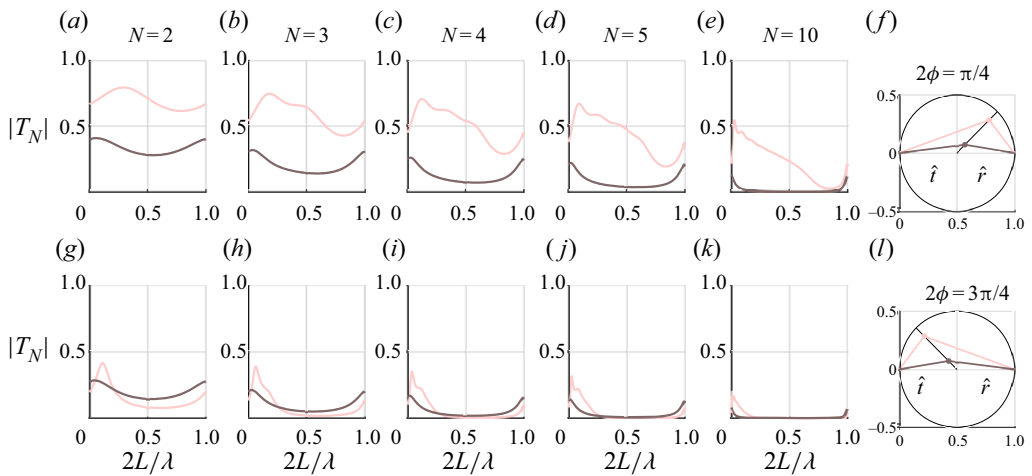
Figure 12. Transmission coefficient magnitude for a set of N equally spaced rows, with N = 2, 3, 4, 5, 10 , and four parameter options regarding \phi and |\delta| . In each graph, the lighter and darker lines correspond, respectively, to |\delta| = 0.1 (weak energy absorption or dissipation) and |\delta| = 0.4 (strong energy absorption or dissipation). The panels (a–e) and (g–k) are for ‘transmission-dominated’ and ‘reflection-dominated’ interactions, respectively. The four parameter options are represented in panels (f,l). See also figure 9 for the meaning of \phi and |\delta| .
