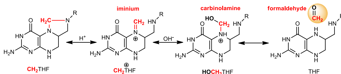
Fig. 1 Hydrolysis reaction of N 5 ,N 10 -methylene tetrahydrofolate as a source of formaldehyde. The cyclic form of CH 2 THF is activated by protonation leading to the iminium species (CH 2 THF + ). This iminium is potentially in equilibrium with its carbinolamine counterpart (HOCH 2 THF). The carbinolamine intermediate can readily decompose into THF and formaldehyde (CH 2 O) in a reversible reaction 28 . CH 2 O can then serve as a direct source of methylene.
