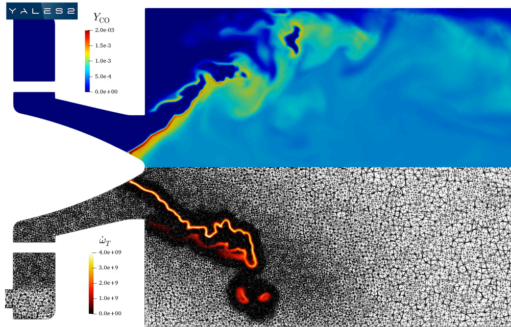
FIGURE 19. Dynamic mesh adaptation in the PRECCINSTA burner test case of Section 6.2 : the instantaneous CO mass fraction and the heat release fields are displayed, together with a slide of the 3D tetrahedral mesh.
