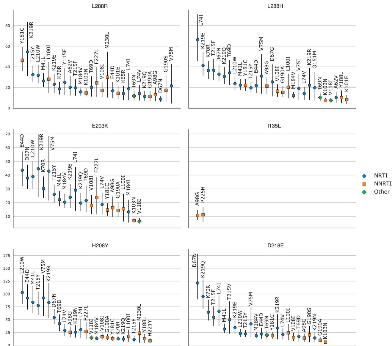
Fig 3. Relative risk of the new mutations with regards to known RAMs on the UK dataset. (i.e. the prevalence of the new mutation in sequences with a given known RAM divided by the prevalence of the new mutation in sequences without this RAM). RRs were only computed for mutations (new and RAMs) that appeared in at least 0.1% (=55) sequences. 95% confidence intervals, represented by vertical bars, were computed with 1000 bootstrap samples of UK sequences. Only RRs with a lower CI boundary greater than 4 are shown. The shape and color of the point represents the type of RAM as defined by Stanford's HIVDB. Blue circle: NRTI, orange square: NNRTI, green diamond: Other. RR values are shown from left to right, by order of decreasing values on the lower bound of the 95% CI.
