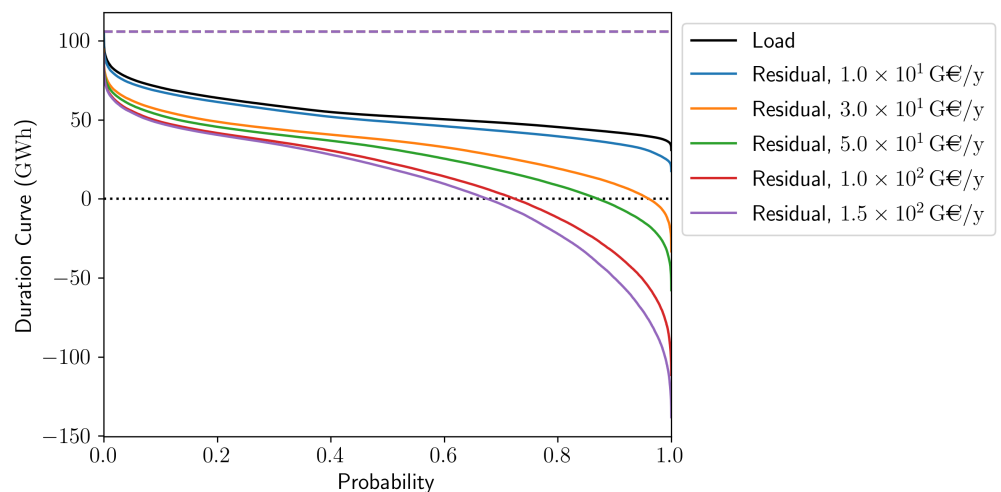
Figure 6. Load duration curve (black) and residual load duration curves (colors) for the optimal solutions of the variable problem at selected values of the expected system total cost without variable renewable energy. The dashed line represents the total installed dispatchable capacity, x_{D_i} .
