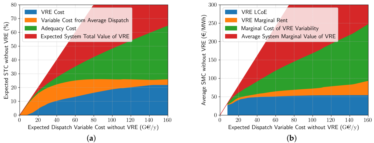
Figure 9. (a) Decomposition of the expected system total cost without Variable Renewable Energy (VRE). The blue and the orange areas, respectively, represent the VRE fixed cost (Equation (2)) and the variable dispatch cost due to the average residual load and add up to the constant version of the expected System Total Cost (STC, second term in Equation (16)). The green area is filled between the constant and the variable versions of the expected STC and represents the adequacy cost (Equation (17), third term in Equation (16)). Finally, the red area is filled between the variable version of the expected STC and the expected STC without VRE and thus represents the expected system total value of VRE (Equation (16)). (b) Decomposition of the average System Marginal Cost (SMC) without VRE. The blue area represents the VRE levelized cost of electricity (Equation (19), last term in Equation (22)). The orange area represents the value of the VRE marginal rent (Equation (20), third term in Equation (22)). The green area represents the marginal cost of VRE variability (second term in Equation (22)). Finally, the red area is filled between the variable version of the average SMC and the average SMC without VRE and thus represents the average system marginal value of VRE (Equation (22)).
