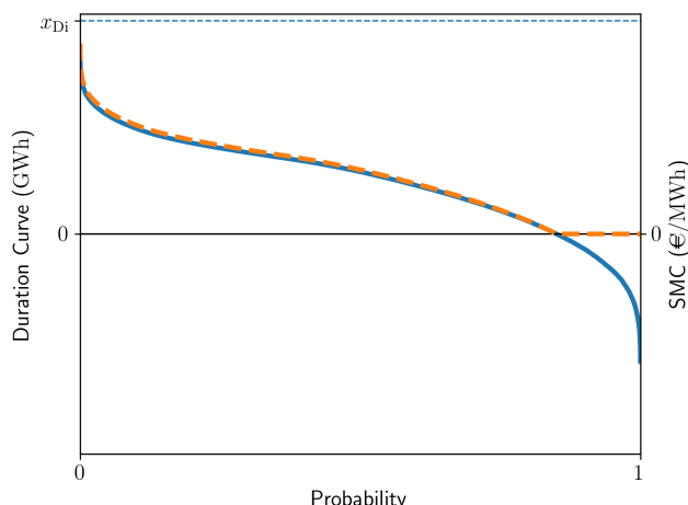
Figure 1. Illustration of the system marginal cost (thick dashed orange line) dependence on the residual load (thick plain blue line) expressed by Equation (9) for an optimal solution. The load is represented as an load duration curve. That is, the load values are ranked by decreasing values and given as a function of the probability that the load exceeds a particular load value.
