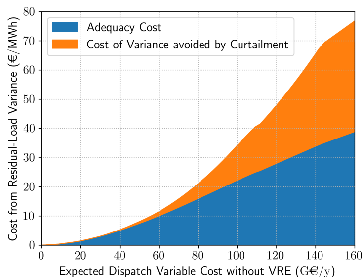
Figure 10. Average variable dispatch cost due to the variance of the residual load with (blue) and without (orange) the reduction by curtailment.
