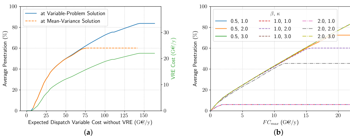
Figure 11. (a) Average penetration (Equation (26)) (left y -axis) versus the expected system total cost without Variable Renewable Energy (VRE) for numerical approximations of the optimal solutions to the variable problem (Equation (4)) (blue) and to the mean-variance problem (Equation (27)) with \kappa = 2 and \beta = 1 (orange). The latter is represented by a plain line when the VRE rental cost constraint is active (when its multiplier is positive) and by a dashed line when it is not. (b) Average penetration (left y -axis) versus the maximum VRE rental cost for numerical approximations of the optimal solutions to the the mean-variance problem (Equation (27)) for different values of \kappa and \beta (orange). For \kappa = 1 and 3 , the curves for different values of \beta overlap.
