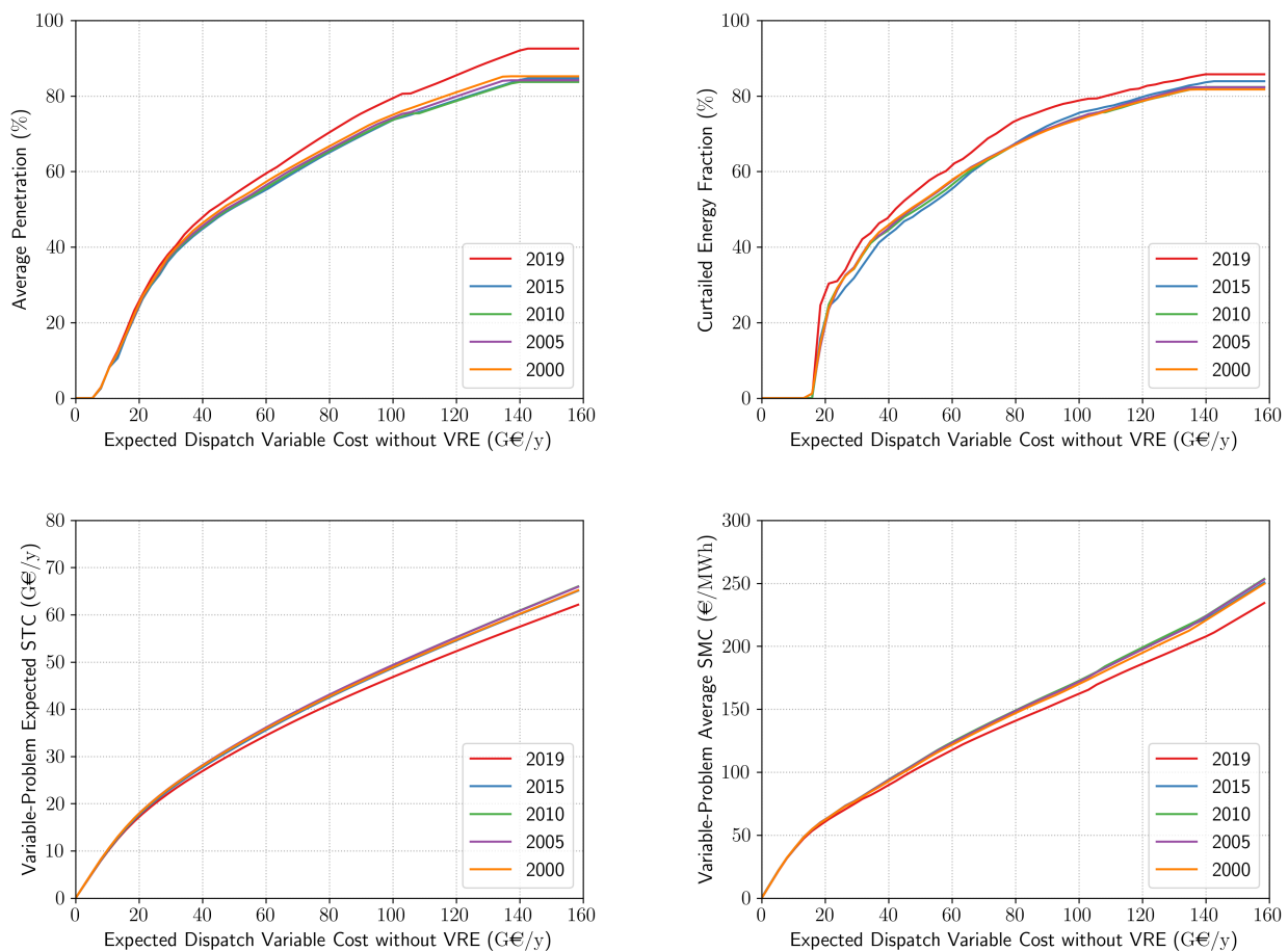
Figure A1. Average penetration ( top left ), fraction of energy curtailed ( top right ), expected system total cost ( bottom left ), and average system marginal cost ( bottom right ) for optimal solutions to the variable problem versus the expected system total cost without variable renewable energy using time series starting in 2019, 2015, 2010, 2005, or 2000 and finishing in 2020.
