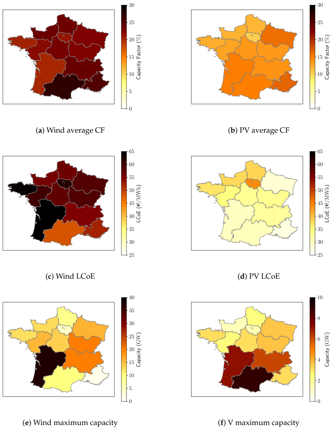
Figure 3. Regional distributions of the (top) average capacity factors, (middle) levelized costs of electricity (Equation (8)), and (bottom) maximum capacities, for onshore wind (left) and photovoltaic (right).
