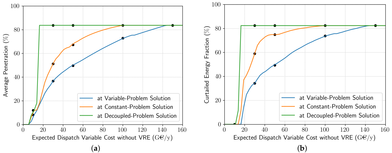
Figure 4. (a) Average penetration (Equation (26)) versus the expected system total cost without variable renewable energy, \mathbb{E}(\overline{\text{STC}}(0)) = T_0 \langle \alpha L^2 \rangle , for numerical approximations of the optimal solutions to the variable problem (Equation (4)) (blue), the constant problem (Equation (14)) (orange), and the decoupled problem (Equation (11)) (green). The black dots indicate—here and in the following plots—the values of these metrics for selected values of the expected system total cost without variable renewable energy, i.e., 10, 30, 50, 100 and 150 G€/y. (b) Corresponding fraction of energy curtailed.
