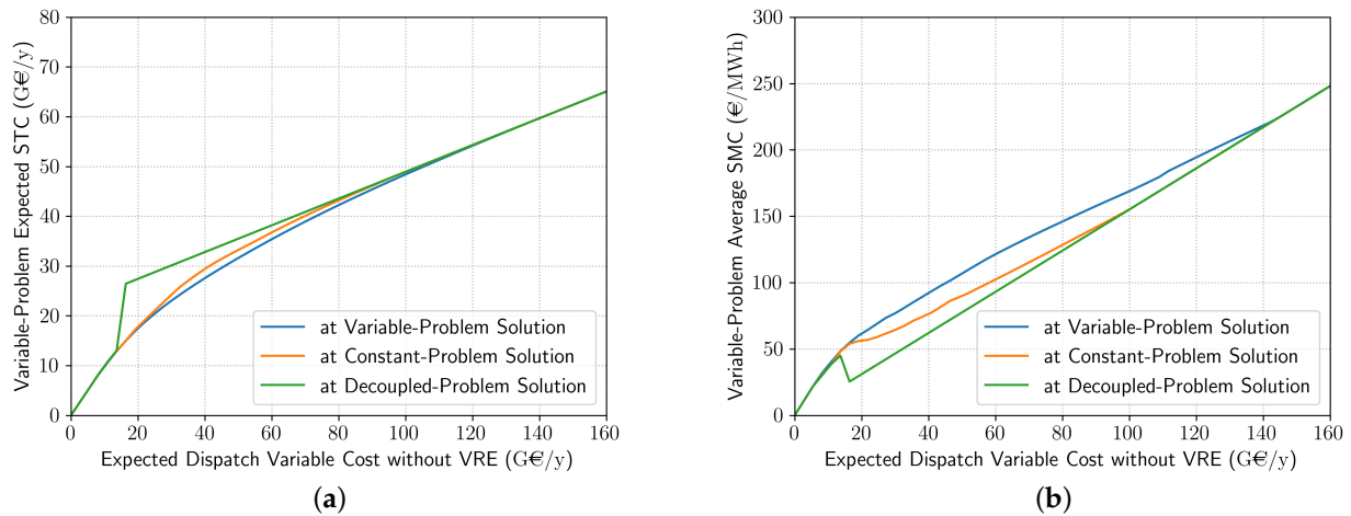
Figure 5. (a) Variable version of the expected system total cost (Equation (3)) for optimal solutions to the variable problem (blue), the constant problem (orange), and the decoupled problem (green). (b) Variable version of the average system marginal cost (Equation (9)) for optimal solutions to the variable problem (blue), the constant problem (orange), and the decoupled problem (green).
