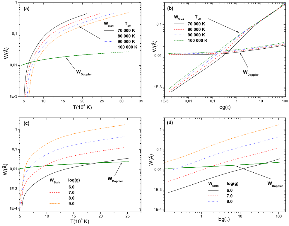
Fig. 2. Stark W_{\text{Stark}} and Doppler W_{\text{Doppler}} widths for the Br VI line 4s^2\ ^1S_0-4s4p\ ^3P_1^o ( \lambda = 95.825\ \text{nm} ) for the atmospheric models of Wesemael (1981) with effective temperatures T_{\text{eff}} = 70\,000\text{--}100\,000\ \text{K} and \log g = 8 as a function of atmospheric layer temperatures (panel a) and as a function of the Rosseland optical depth (panel b), and for the atmospheric models of Wesemael (1981) with \log g = 6\text{--}9 and effective temperature T_{\text{eff}} = 80\,000\ \text{K} as a function of atmospheric layer temperatures (panel c) and as a function of the Rosseland optical depth (panel d).
