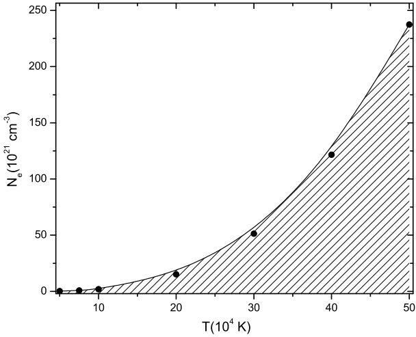
Fig. 1. Temperatures and densities at which a plasma is treated as ideal.
