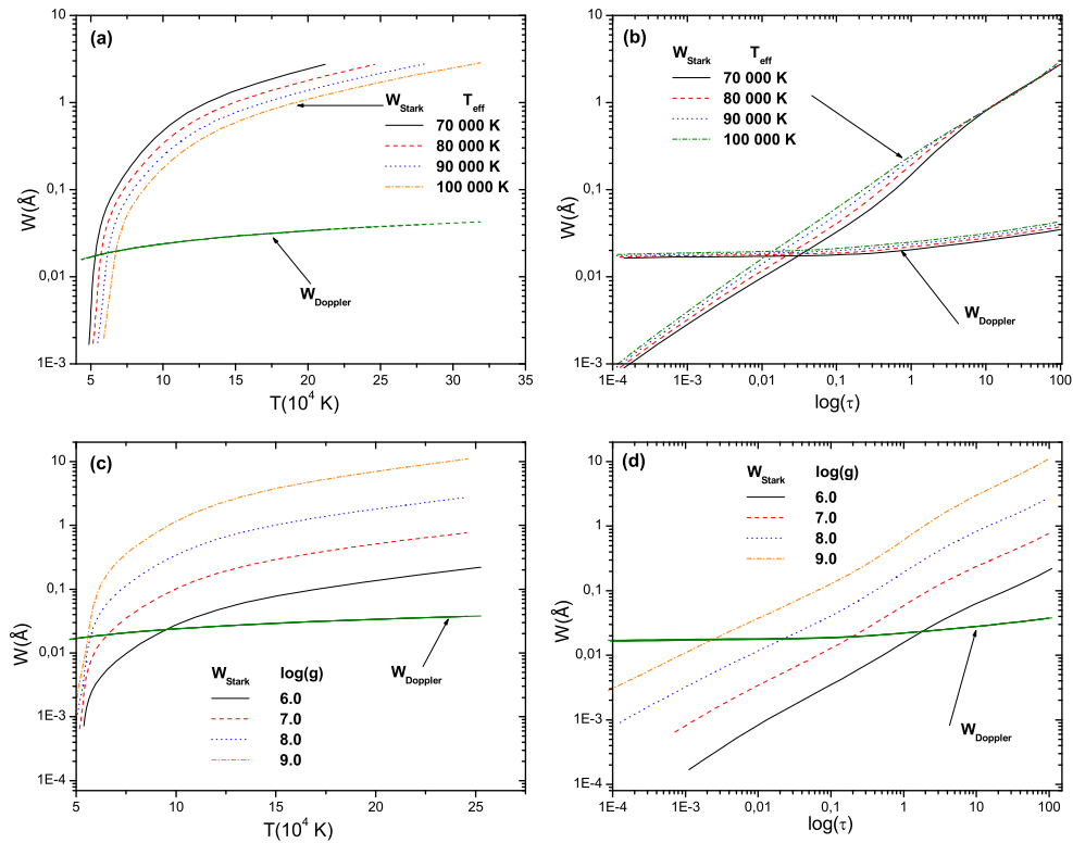
Fig. 3. Same as in Fig. 2 but for the Kr V line 4s^24p5s\ ^1P_1^o-4s^24p5p\ ^1S_0 ( \lambda = 176.4478\ \text{nm} ).
