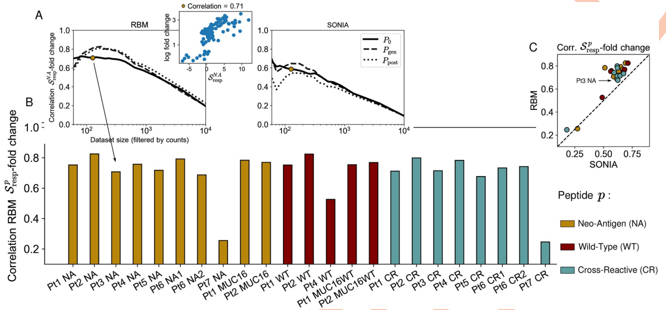
Fig 3. Model scores of T-cell clonal expansion. A: The RBM calculated response scores S_{\text{resp}}^p for each TRB clone in each antigen-stimulation condition p . The correlation between the S_{\text{resp}}^p and clone fold change is poor when considering all clones, as low-count clones are a source of noise. A significant correlation is recovered by progressively filtering out the low-abundance sequences from the testing set, shown on the example of stimulation by p = \text{NA} of Pt3 PBMC. For both RBM and SONIA (shown on the right), the correlation is robust to the choice of different background distributions: P_0 (the probability learned on the same patient’s dataset at day 0), P_{\text{gen}} (the probability of generating a given CDR3, described by OLGA [21]) and P_{\text{post}} (the post-thymic selection CDR3 distribution, sampled here from a default human TRB model available in SONIA [15]). The small differences between the 3 curves are mainly due to sampling, see also Materials and methods . B: The correlation coefficient between the RBM S_{\text{resp}}^p and clone fold change for each antigen-stimulation experiment p (color-coded by antigen) when retaining the 125 most abundant clones (the golden dot in panel A). Data from [16] correspond to p = \text{NA, CR, WT, MUC16, MUC16WT} (Pt1, Pt2), p = \text{NA, CR} (Pt3, Pt5, Pt7), p = \text{NA, CR, WT} (Pt4), p = \text{NA1, CR1, NA2, CR2} (Pt6), see also Table 1 . C: Scatter plot comparing S_{\text{resp}}^p from the RBM and SONIA.
