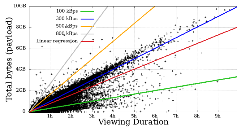
Figure 14. Bytes throughput per second of mobile users on the system in the broadcast Impeachment start session— Camara dos Deputados .
