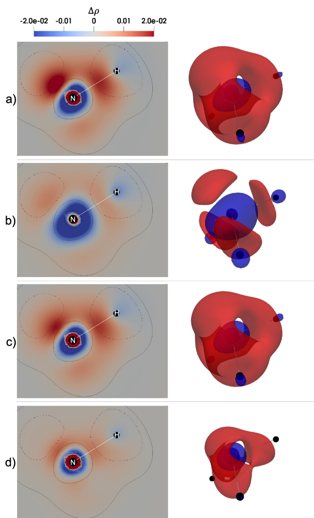
Figure 7. Plots of the difference in electron density between HF and DFT methods for a) IM, b) Cry, c) \text{XCW}_{\lambda=0.001} and d) \text{XCW}_{\lambda=0.030} for ammonia molecule ( \Delta\rho = \rho(\mathbf{r})_{\text{HF}} - \rho(\mathbf{r})_{\text{DFT}} ). Isosurfaces with negative values ( -0.005 a.u.) in blue and positive values ( 0.005 a.u.) in red. Contours in plots with the isovalues 0.5 (continuous black line) and 0.9 (dotted black line) of the ELF in Cry.
