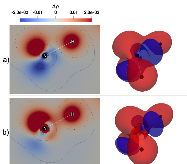
Figure 6. Plots in 2D and 3D of \rho difference between Cry and XCW for a) HF and b) DFT ammonia molecule calculations ( \Delta\rho = \rho_{\text{Cry}} - \rho_{\text{XCW}} ). Contours with the isovalues 0.5 (continuous line) and 0.9 (dotted line) of ELF in Cry. Isosurfaces with negative values ( -0.005 a.u.) in blue and positive values ( 0.005 a.u.) in red.
