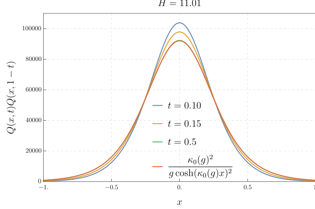
Figure S11. Optimal noise profile \tilde{h}(x, t)/g = Q(x, t)Q(x, 1 - t) as a function of x for H = 11.01 and various times t . A weak time dependence can be seen. For t = 1/2 (in green) it already overlaps almost perfectly with the "soliton only" (time independent) solution, valid in the boundary layer x \sim 1/\kappa_0 for H \rightarrow +\infty (in red)
