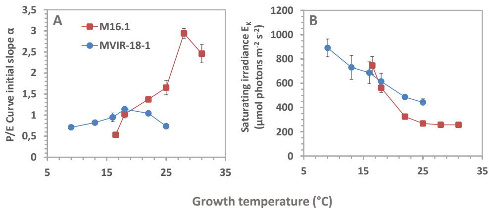
Figure S2: Variations of the initial curve slope \alpha (A) and the saturation irradiance (B) using 480 nm light, in Synechococcus spp. M16.1 (red) and MVIR-18-1 (blue).
