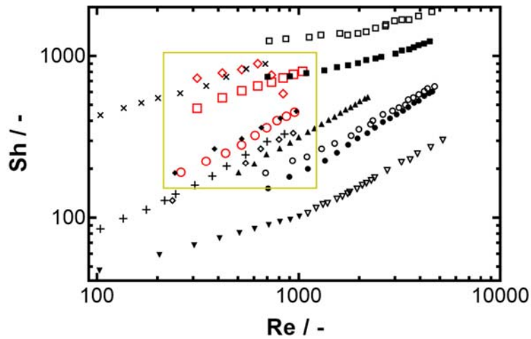
Fig. 7. Logarithmic representation of Sherwood number versus Reynolds number from experimental data from this work for no mesh promoter and no gas flow ( \circ ), medium mesh size at ADE pressure of 3.0 bar ( \square ), and no mesh promoter with ADE pressure of at 4.0 bar ( \diamond ). These results are compared with data from previous reports for electrochemical cells that consider rectangular flow channel cells in the presence and absence of a mesh promoter as adapted from [38]: nickel solid electrode: ( \bullet )no mesh promoter and ( \circ ) with a mesh promoter. Nanostructured nickel deposit: ( \blacksquare ) no mesh promoter and ( \square ) with a mesh promoter. Nickel electrode in the FM01-LC electrolyser: ( \blacklozenge ) no mesh promoter and ( \diamond ) with a mesh promoter.
