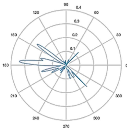
Fig. 7: Diffraction coefficient of a sea patch
