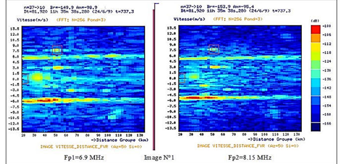
Fig. 8: Velocity - Doppler image for HF radar in a monostatic configuration
