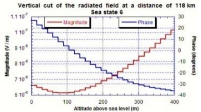
Fig. 5: Incident field at the target location
