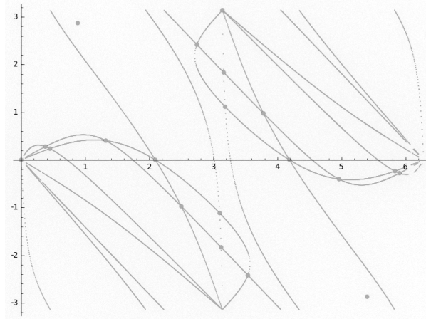
FIGURE 3. Points on the torus (axis are the arguments of x and y ). The singular points, represented by a small disc, are all intersection of 1-dimensional branches but two that are isolated.
