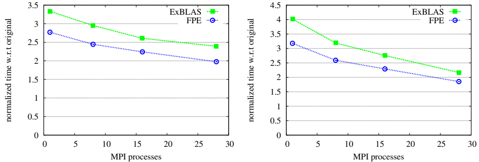
Fig. 3: Strong scaling results of the original and reproducible PBiCGStab variants with the Jacobi preconditioner on one SkyLake node for the s3dkq4m2 (left) and af_shell10 (right) matrices, see Tab. 1 for details.
