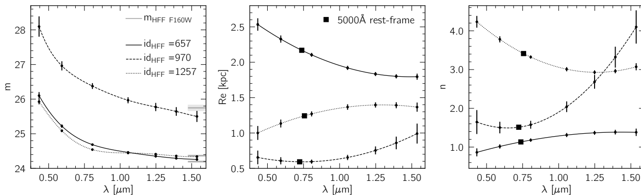
Figure 4. Example fitting results of the apparent magnitude ( m ), effective radius ( R_e ), and Sérsic index ( n ) as a function of wavelength for three galaxies in the Abell1063 parallel field, all at roughly the same redshift. These three galaxies, are chosen to display the variety of functional forms that can be fit for different galaxy parameters. For each galaxy, the fit is shown in a different line style as indicated in the legend and the black squares indicate the 5000\text{\AA} rest-frame values that can be read from the Chebyshev polynomials. The left panel shows the apparent magnitude of each object, as derived by GALFITM, with the F160W magnitude from the HFF-DeepSpace catalogue (Shiple et al. 2018) indicated as a horizontal grey line around 1.6\mu\text{m} , where the uncertainty is shown as a shaded grey region. Although these H-band magnitudes are measured with different methods, they are consistent, indicating that the modelling is reliable, even for faint objects, such as galaxy \text{id}_{\text{HFF}} = 970 . In the modelling, the magnitudes are allowed to vary freely as a function of wavelength (hence, rest-frame magnitudes are not derived directly from the Chebyshev polynomial), while for the size and Sérsic index of each galaxy, which are shown in the middle and right panel, the Chebyshev polynomial fit is allowed to vary as a second order polynomial. All of the errors shown are the ones derived by GALFITM and are therefore underestimated by a factor of 2 to 2.5 (see §4). The magnitude errors are increased by a factor of 5, to illustrate that the faintest galaxy has the largest uncertainties.
