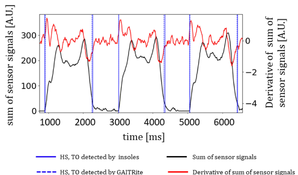
Figure 1. Detection of HS and TO events by the insoles and GAITRite®.
