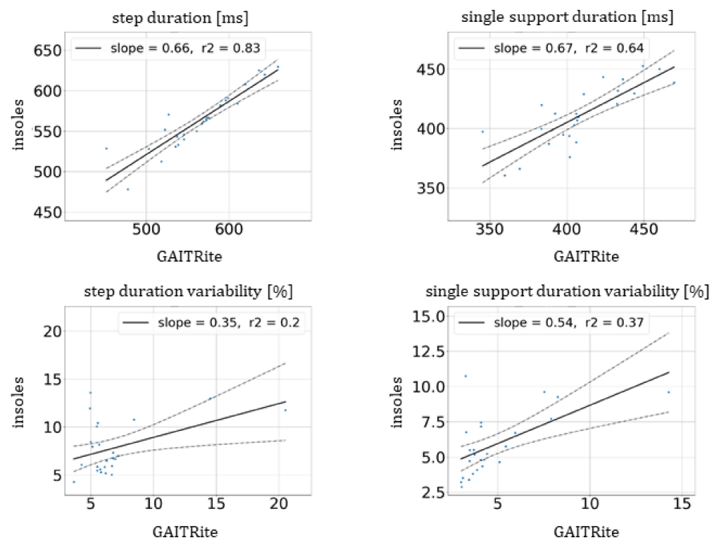
Figure 5. Linear regression of average estimates and estimates of variability of bipedal gait parameters with step duration and single support duration between GAITRite ® mat and the insoles (solid lines). The dashed lines represent the confidence region. The values of the slope and the coefficient of determination, r^2 , are provided in the legends.
