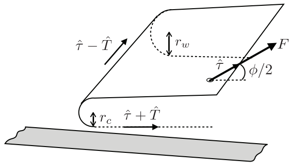
FIG. 9. Geometry of the fold as bending energy is taken into account. The fold is assumed to have a conical shape, with a radii of curvature r_c and r_w at the fracture tip and at the free end, respectively.
