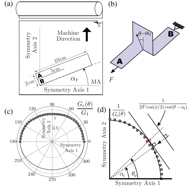
FIG. 7. a) The sample dimensions and its orientation with respect to the material axis (Axis-1) and the machine direction (Axis-2). b) Trouser test configuration for the measure of the fracture energy G_c(\theta) as function of the fracture direction \theta . c) The Polar plot of the fracture energy as a function of \theta . The solid line is the best fit to the experimental data of the form G_c(\theta) = G_1 \cos^2(\theta) + G_2 \sin^2(\theta) . Values of G_1 = 6.0 \text{ kJ/m}^2 and G_2 = 5.3 \text{ kJ/m}^2 . d) The Wulff’s type diagram G_c^{-1}(\theta) construction leads to find graphically the direction of propagation \theta_w , as the first intersection point (indicated by a red circle), and the force F required for a given tearing direction \alpha_t .
