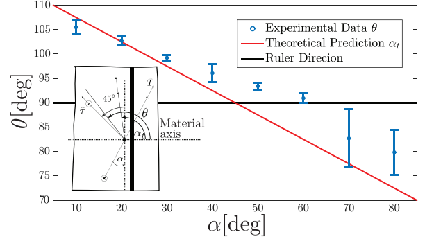
FIG. 5. Angle of fracture propagation \theta as function of the position of the pulling point (orientation of grip vector \alpha ) for a fixed pulling angle of 45^\circ with respect to the ruler. Red line indicates crack orientation as predicted by the tearing vector (3). Horizontal black line depicts the ruler orientation. Inset: Sketch of the geometry of the experiment.
