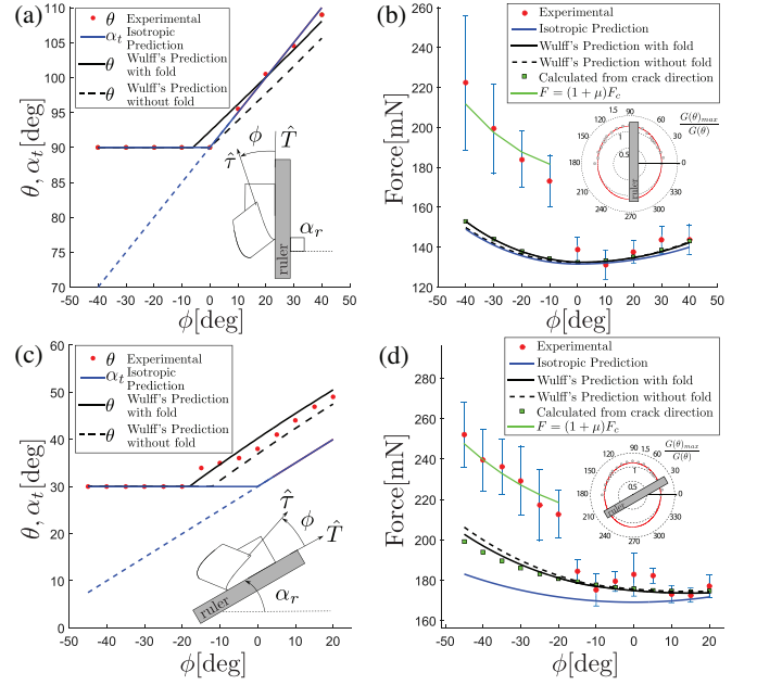
FIG. 6. Angle of fracture \theta and tearing force F as function of \phi (measured with respect to the ruler). a) and b) ruler oriented at 90^\circ with respect to the film axis. c) and d) ruler oriented at 30^\circ with respect to the film axis. In a) and c) predictions from geometrical arguments, \theta = \alpha_t , (without ruler constrain) are represented by straight blue lines. For \phi < 0 , solid horizontal blue lines indicate propagation along the ruler, \theta = \alpha_r . Below these lines, no fracture propagation can occur due to the presence of the ruler. Dashed black lines are the predictions including anisotropy (Wulff's without fold), whereas solid lines include in addition the effect of the fold stiffness. In b) and d) geometrical model predictions for the tearing force from Eq. 2 are indicated with blue lines. When fracture is guided by the ruler, \theta = \alpha_r , the tearing force is given by Eq. 4. Dashed black lines indicate corrections due to fracture anisotropy (Wulff's plot) while solid black lines indicate predictions including both, anisotropy and fold effects. Insets in b) and d) indicate the inverse of fracture energy as a function of the propagation angle \theta , and the ruler orientation.
