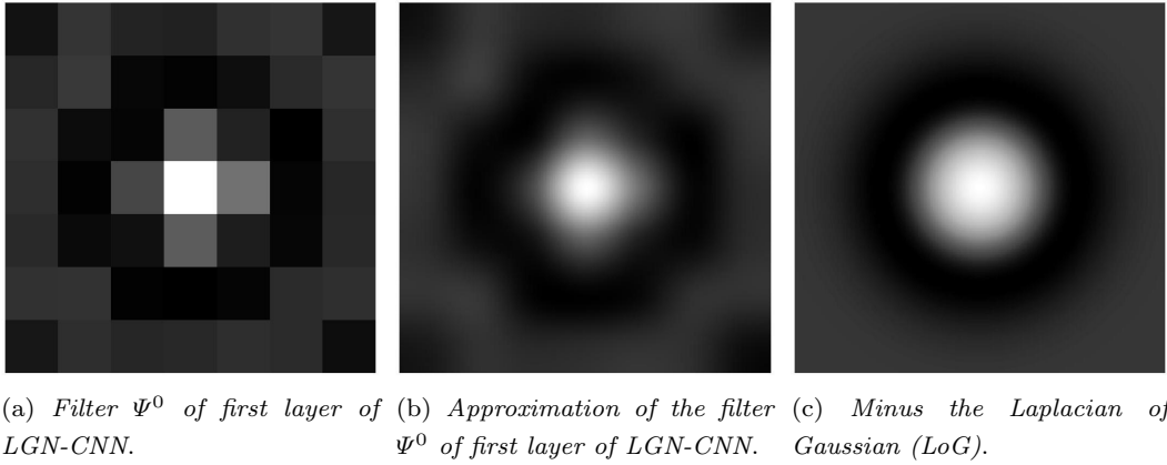
Fig. 6: The first figure shows the 7 \times 7 filter \Psi^0 of the neural network. To better visualize the filter \Psi^0 , we provide an approximating 280 \times 280 filter and minus the LoG.
