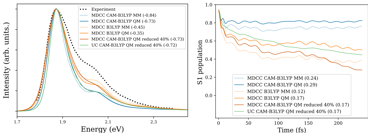
FIG. 6. Using molecular dynamics cross-correlation (MDCC) for bath correlation ( \tilde{\mathcal{J}}_{\text{cross}} ), different functionals and solvent models strongly influence the energy gap between electronic states. This can dramatically increase fast non-adiabatic transitions from the S_1 state and increase shoulder intensity. Lineshapes have been shifted by the left legend value to match experiment in eV. Legend values on the right are the average gap \omega_{12}^{\text{av}} in eV.
