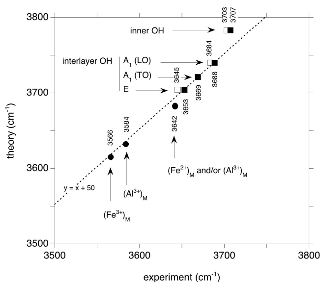
Figure 5. Relation between the theoretical frequencies (Fig. 1) and experimentally observed vibrational bands. Open squares: FTIR spectrum of Monte Fico lizardite (Balan et al., 2002); full squares: Raman frequencies of Monte Fico lizardite (Compagnoni et al., 2021). Black circles: signals ascribed to cationic impurities in the vibrational spectra of the Monte Fico and Lz1 lizardite. The average value of theoretical frequencies related to (\text{Fe}^{2+})_{\text{M}} ( 3683 \text{ cm}^{-1} ) almost coincides with the higher-frequency contributions related to \text{Al}^{3+} cations ( 3682 \text{ cm}^{-1} ). The theoretical model overestimates the experimental stretching frequencies of interlayer-OH groups by \sim 50 \text{ cm}^{-1} .
