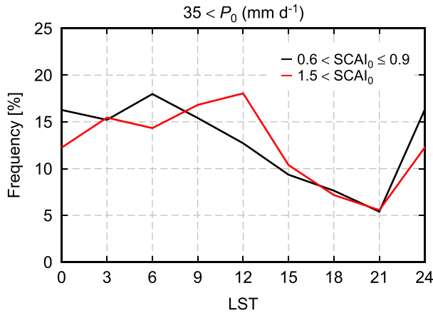
FIG. 9. A 3-hourly histogram of the precipitation peaks of P_0 > 35 \text{ mm day}^{-1} as a function of local time for the more-aggregated case ( 0.6 < \text{SCAI}_0 < 0.9 ; in black) and less-aggregated case ( \text{SCAI}_0 > 1.5 ; in red).
