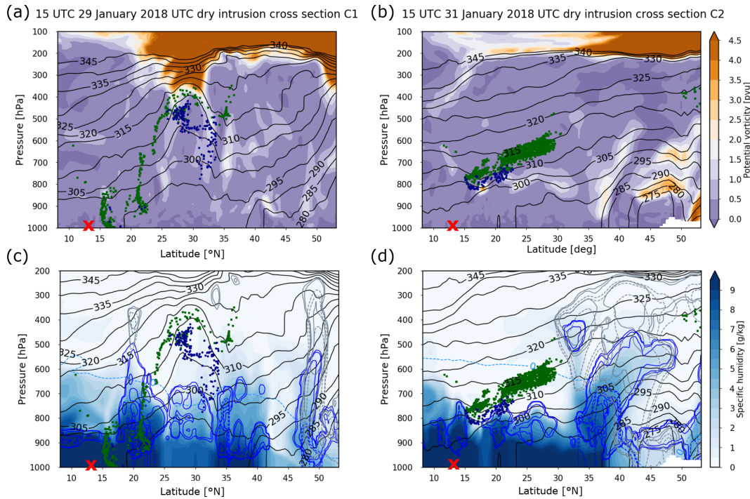
Figure 14. Meridional cross-sections along the lines C1 and C2 in Fig. 11b at 15:00 UTC on 29 January 2018 through the upper-level cut-off (C1; a, c ) and at 15:00 UTC on 31 January 2018 showing the strongly descending air parcels west of the cut-off (C2; b, d ). Filled contours show ( a, b ) potential vorticity and ( c, d ) specific humidity. Isentropes are shown by black contours every 5 K. In ( c, d ) cloud liquid water is shown by solid blue contours, rainwater by dashed blue contours, ice water content by grey contours and snow water content by dashed grey contours. All hydrometeor contour lines correspond to 5, 10 and 50 \text{mg kg}^{-1} . The green and blue points correspond to the positions of air parcels within \pm 1^\circ longitude of the cross-section. The green air parcels form together the cloud layer (940–700 hPa), and the blue air parcels form the sub-cloud layer (surface to 940 hPa) above Barbados during the period of the extratropical dry intrusion between 1–4 February 2018. The latitude of Barbados is highlighted by the red cross at the surface.
