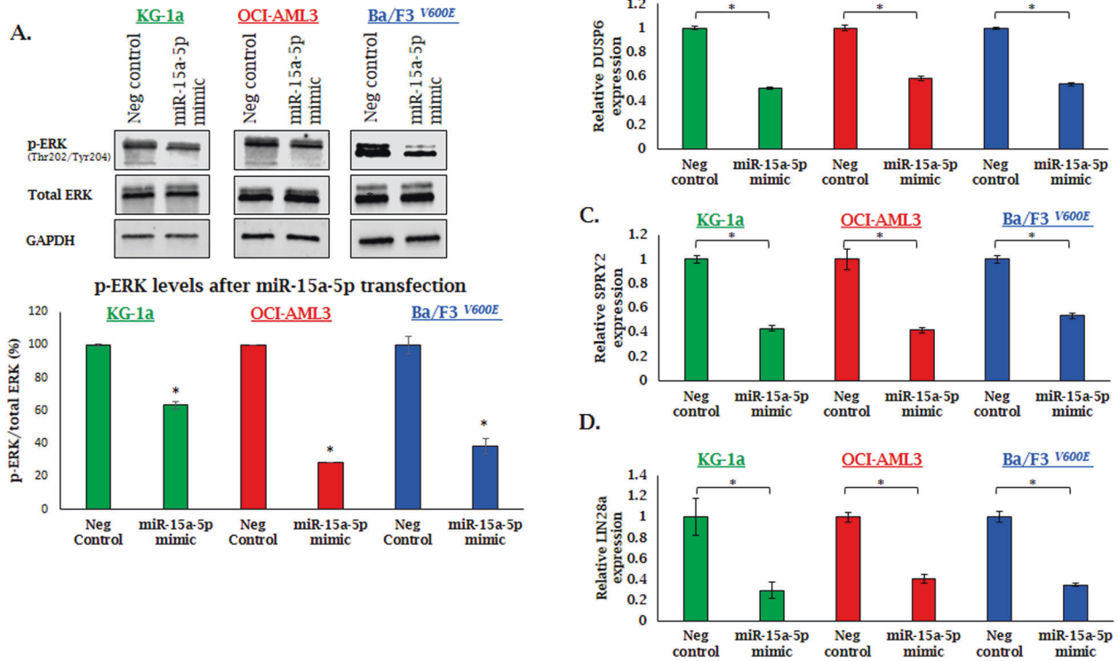
Fig. 3 Protein levels of p-ERK and ERK-cascade target genes after miR-15a-5p transfection. KG-1a, OCI-AML3, and Ba/F3 V600E cells were transfected with a miR-15a-5p mimic (50 nM) or a negative control for 48 h. A p-ERK protein expression levels were downregulated after transfection with a miR-15a-5p mimic in all cell lines. Protein samples were resolved by SDS-PAGE. Antibodies to p-ERK, ERK, and GAPDH (loading control) were used to assay the levels of protein, which were then quantified by the Licor imaging system (bottom graph). The graph presents values from at least 3 experiments. B The expression of DUSP6, C SPRY2, and D LIN28a in KG-1a (green), OCI-AML3 (red) and Ba/F3 V600E (blue) cells post transfection as measured by qRT-PCR from at least 3 experiments. * p < 0.05 .
