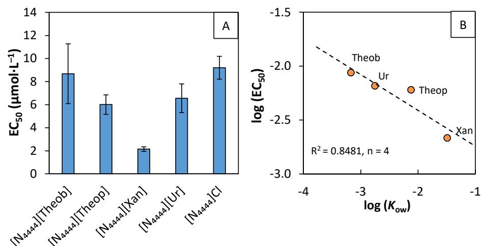
Figure 2. (A) EC_{50} values ( \mu\text{mol}\cdot\text{L}^{-1} ), determined after 96 h of exposure time of Raphidocelis subcapitata to the purine-based salts and [\text{N}_{4444}]\text{Cl} . The error bars correspond to the 95% confidence interval. (B) Correlation between the logarithm of EC_{50} and the logarithm of the octanol–water partition coefficient ( K_{ow} ) of the different salt anions [59]. The coefficient of determination ( R^2 ) and the number of experimental points used for the linear regression ( n ) are also presented.
